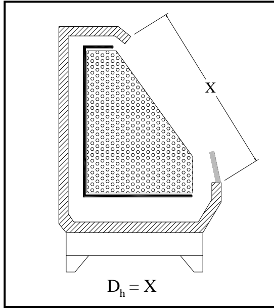
Figure D4: Semi-vertical Open Multi-deck with Transparent Front
