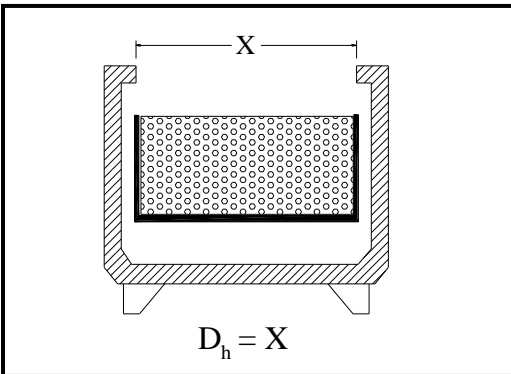
Figure D9: Horizontal Open Single-deck Island
