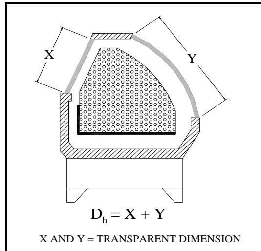
Figure D8: Service Over Counter with Curved Transparent Front
