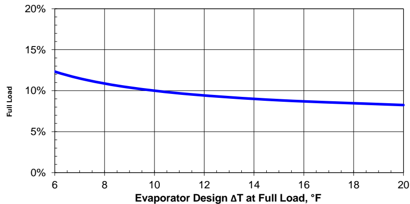
Figure 4. IPLV.IP and NPLV.IP Tolerance (Tol 2 ) Curve
