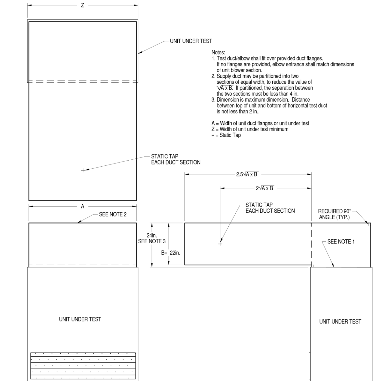
Figure 1. Limited Height Test Chamber Upflow Unit Test Duct
