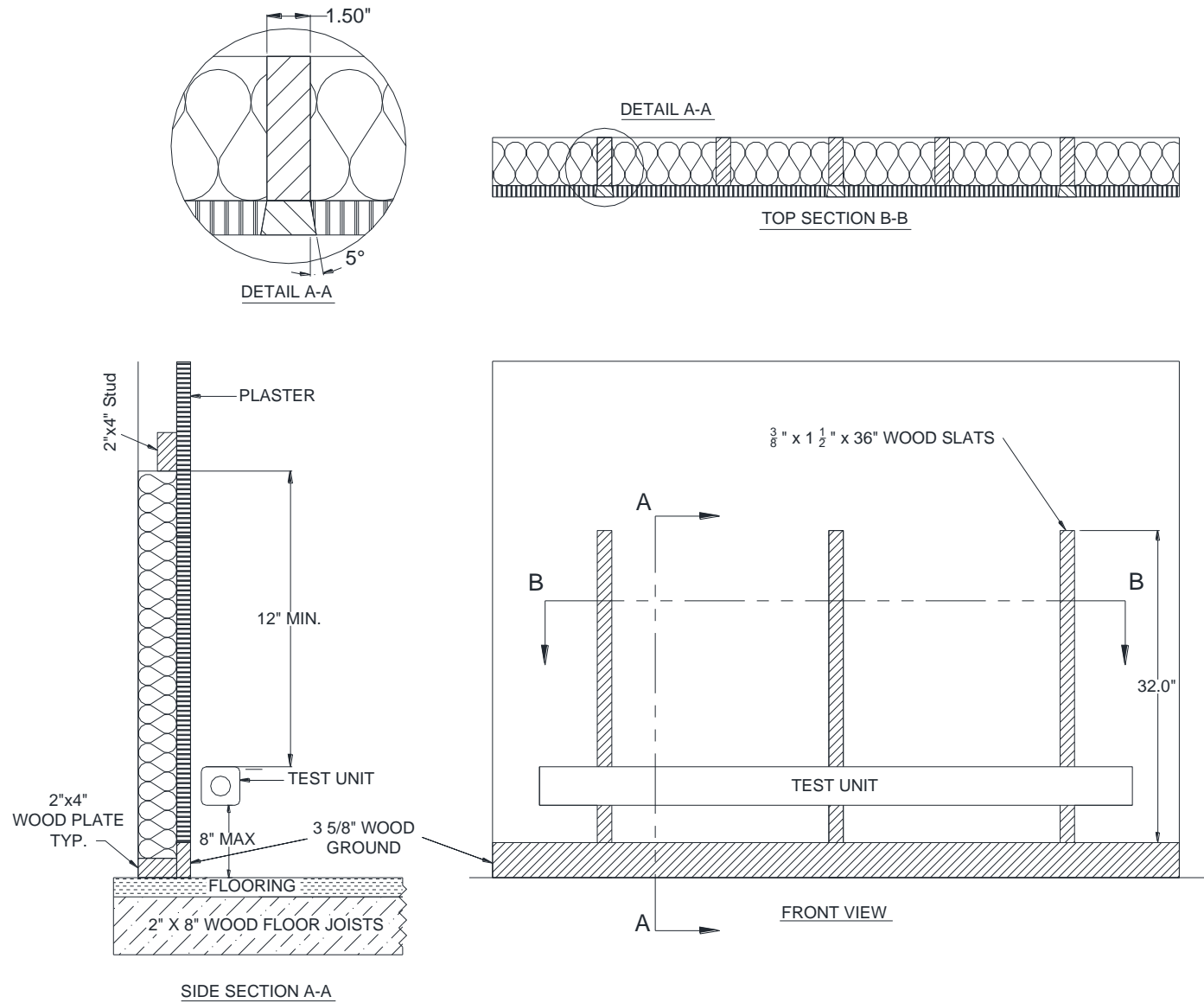
Figure C1. Test Unit Wall Construction
