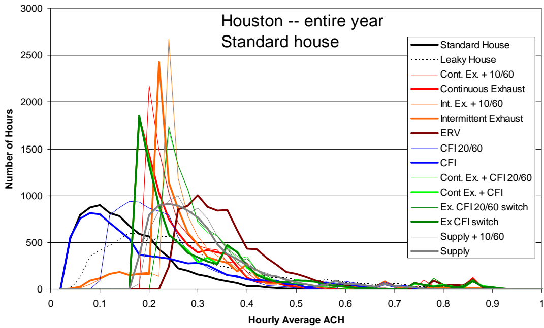
Figure A.27 Frequency distribution of hourly average air change rate (0.02 ach bins) for the entire year in Houston
