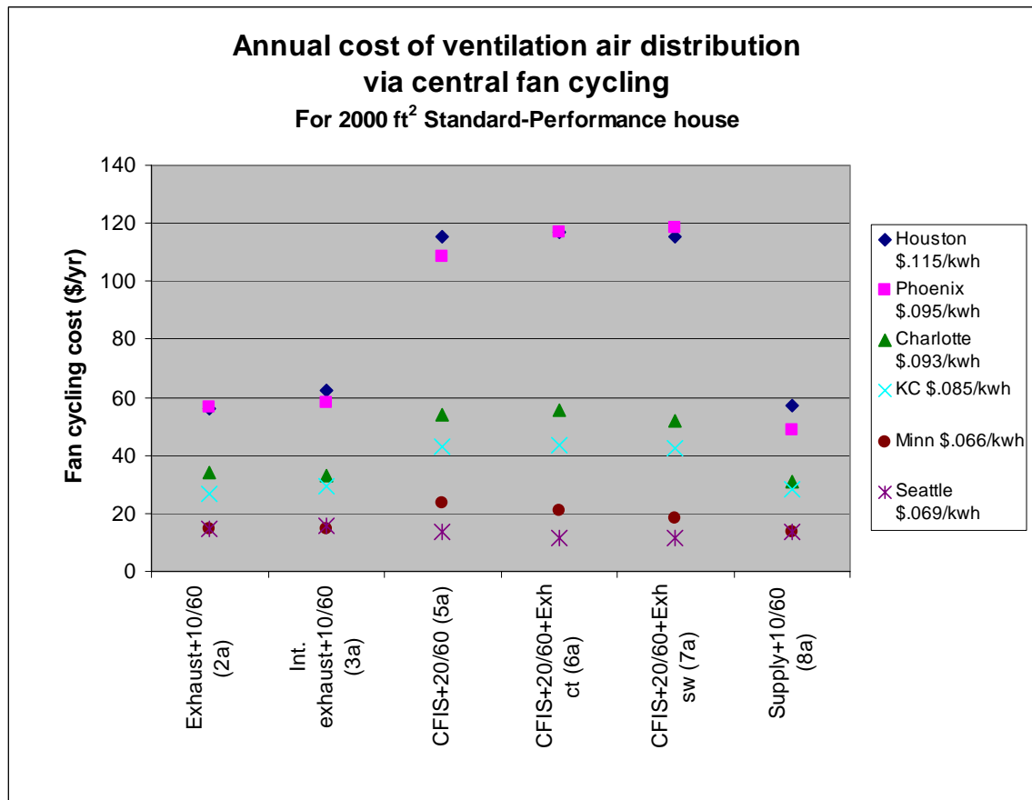
Figure 3.9(a) Annual cost of ventilation air distribution and thermal comfort mixing via the central fan for the Standard-Performance house, for all six climate locations
