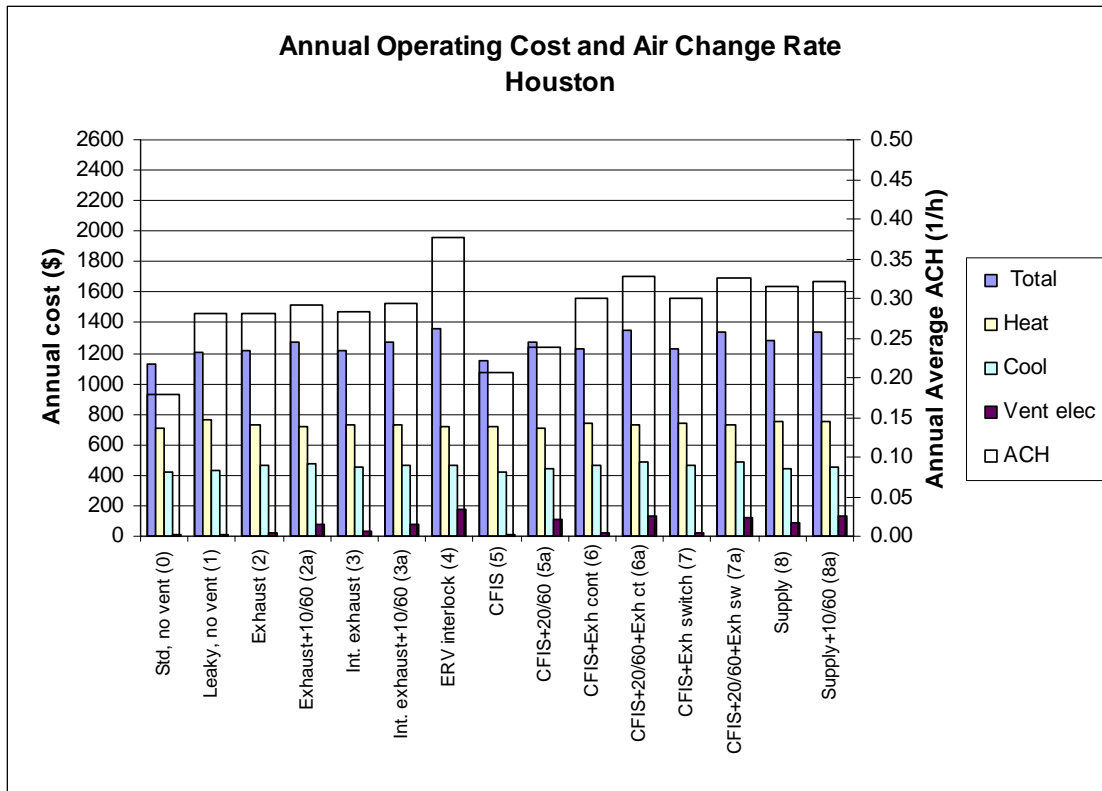
Figure A.1 Annual operating cost and annual average air change rate for Houston
