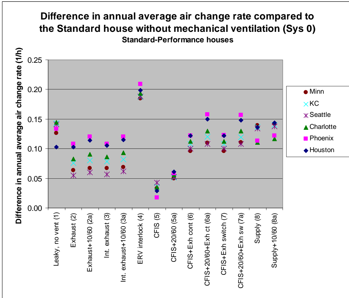
Figure 3.2(a) Difference in annual average air change rate (ach) for Standard-Performance houses compared to the Standard house without mechanical ventilation
