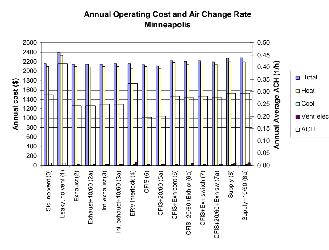
Figure B.11 Annual operating cost and annual average air change rate for Minneapolis
