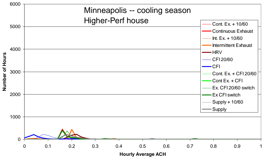
Figure B.41 Frequency distribution of hourly average air change rate (0.02 ach bins) for the cooling season in Minneapolis
