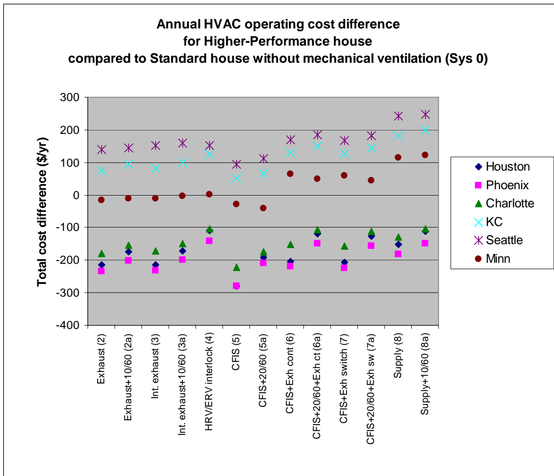
Figure 3.7(b) Annual HVAC operating cost difference for the Higher Performance house compared to the Standard house without mechanical ventilation, for all six climate locations
