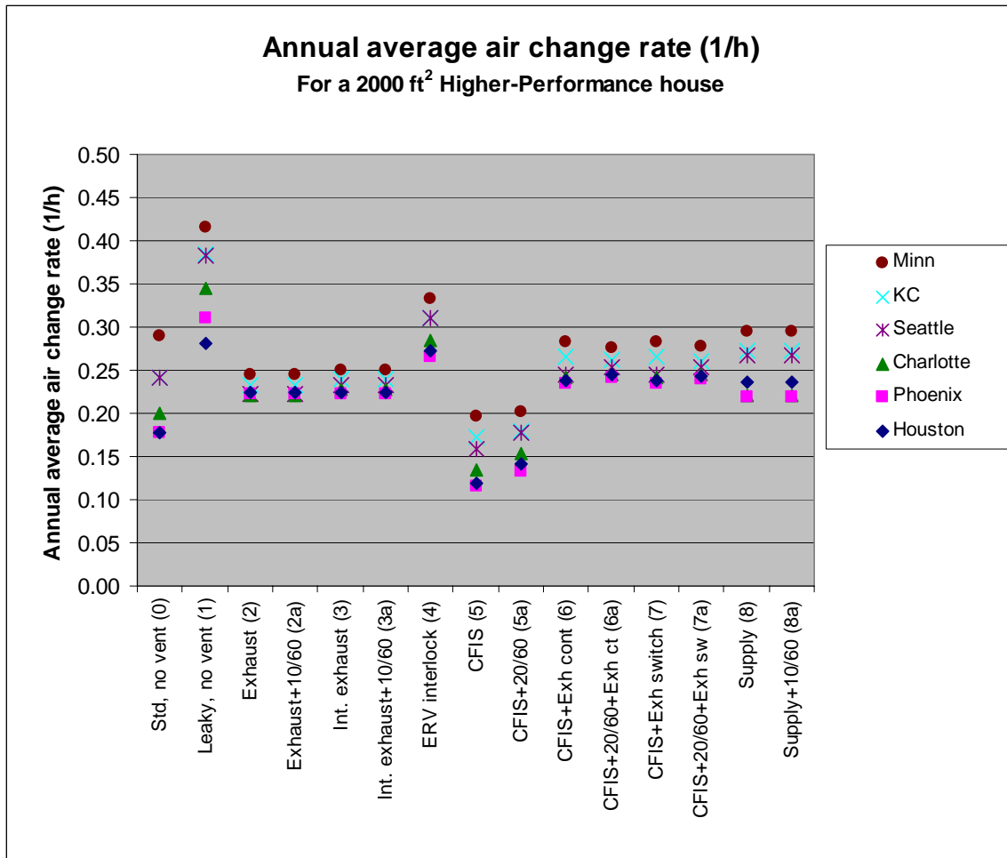
Figure 3.1(b) Annual average air change rate (ach) for Higher-Performance houses (Systems 2 through 8a)
