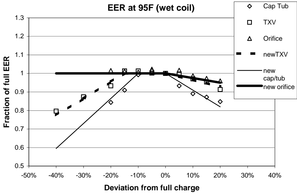
Figure C11. Wet Coil EER variation with charge
