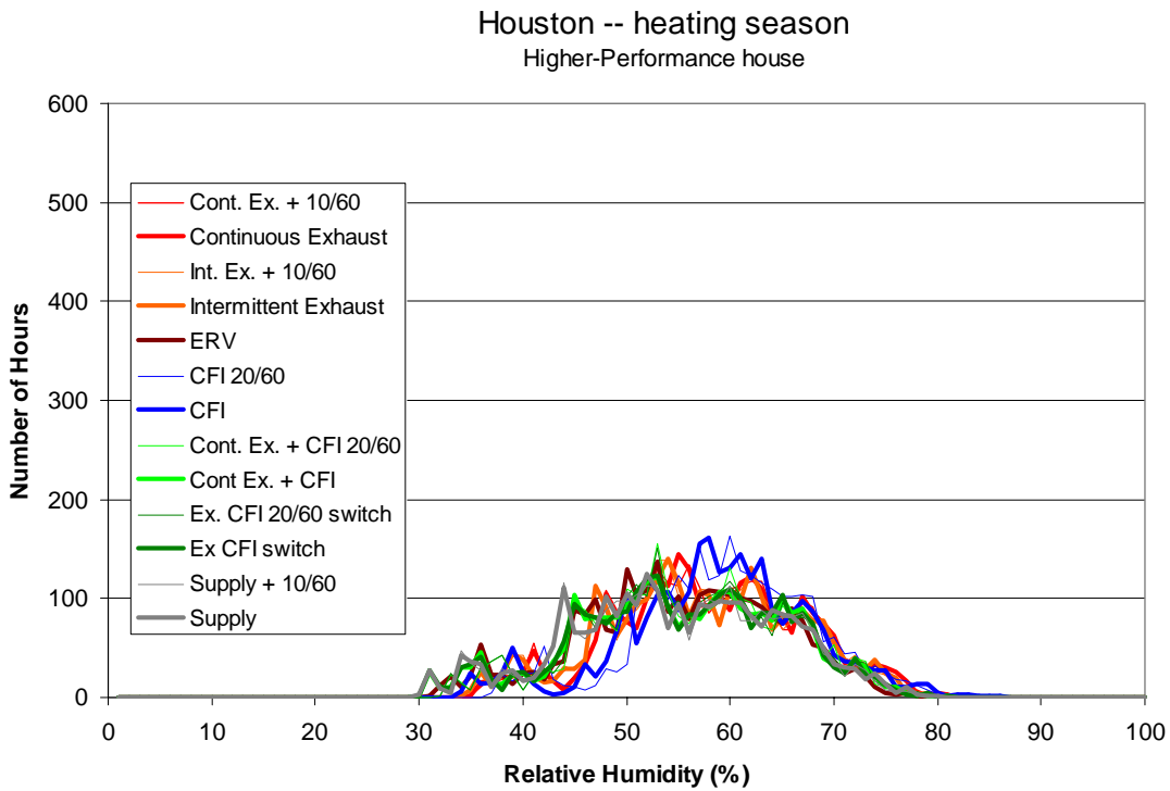
Figure 3.12(b) Frequency distribution of hourly average indoor relative humidity (1% RH bins) for the heating season for the Higher-Performance house in Houston
