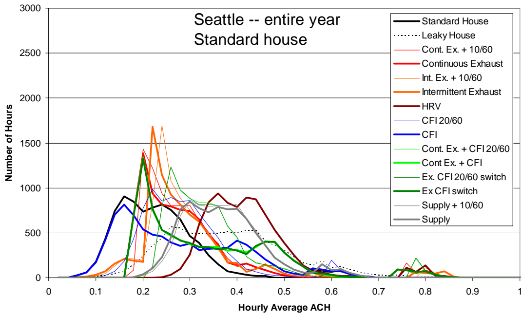
Figure 3.4(b) Hourly average air change rate (ach frequency in 0.02 bins) for Seattle, for Standard-Performance house
