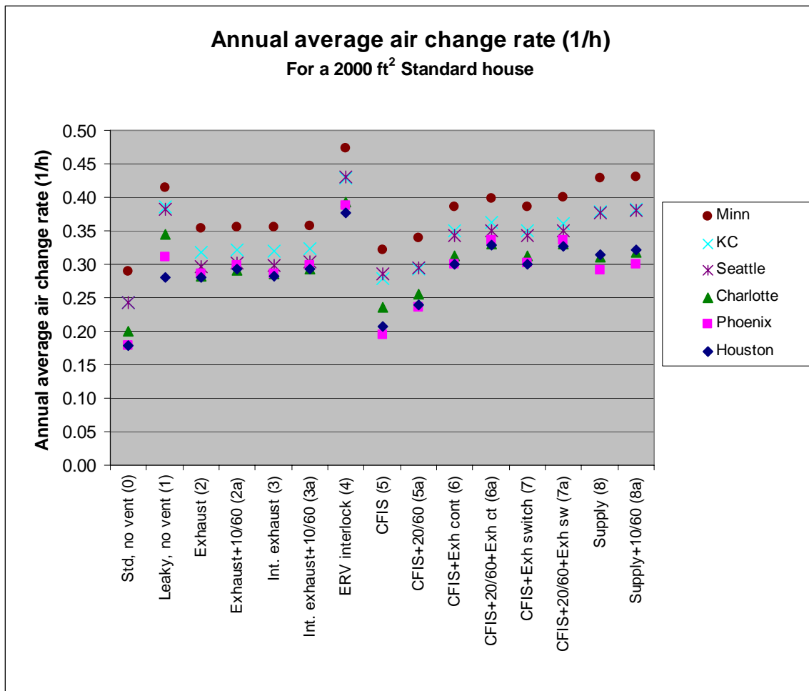
Figure 3.1(a) Annual average air change rate (ach) for Standard-Performance houses
