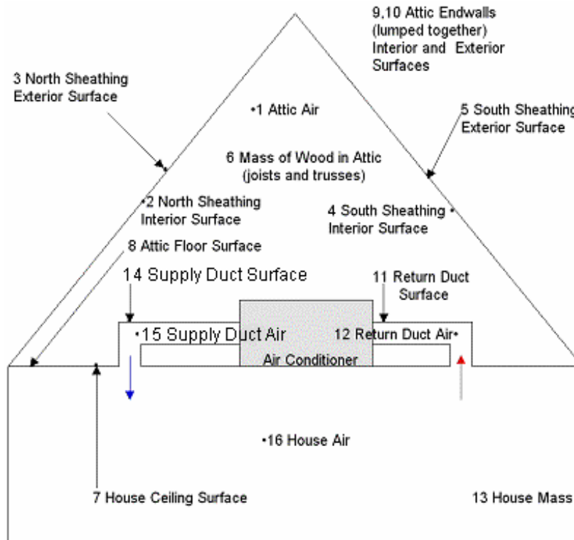
Figure C8: Nodes For Heat Transfer Model
