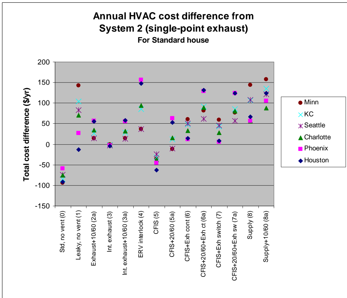
Figure 3.6(a) Total HVAC operating cost difference compared to System 2 (single-point exhaust), for all six climate locations
