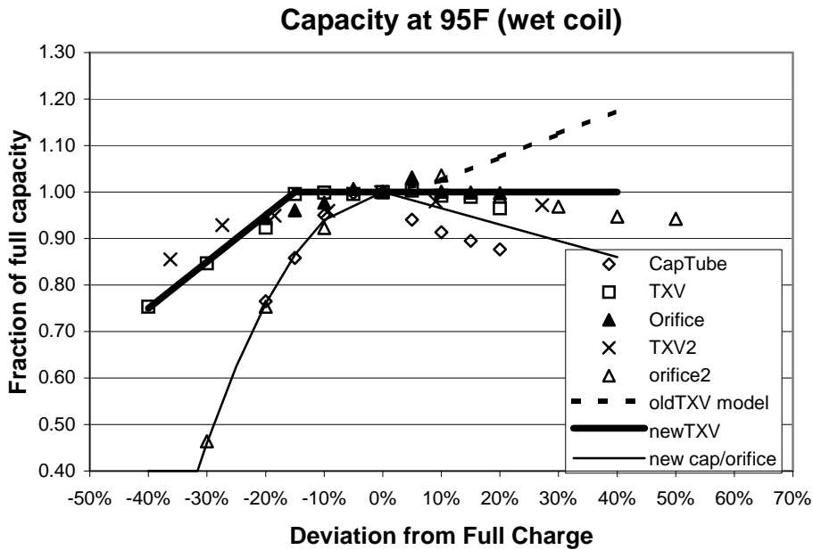
Figure C10. Wet Coil capacity variation with charge
