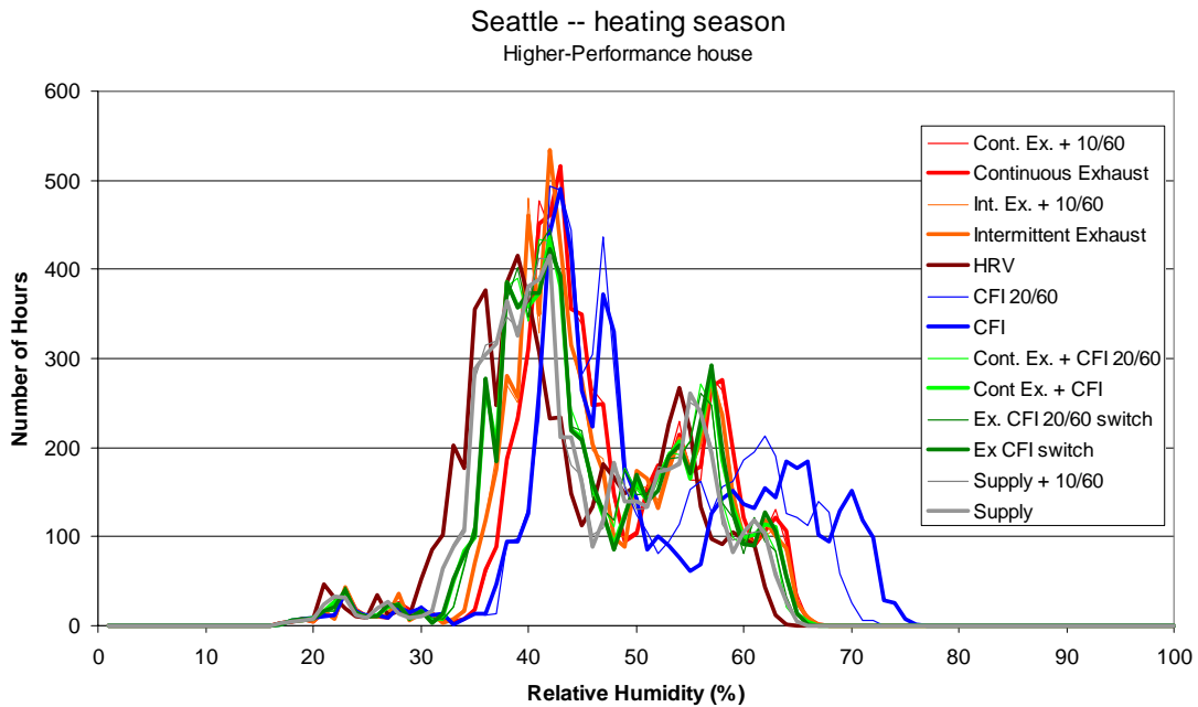
Figure B.24 Frequency distribution of hourly average indoor relative humidity (1% bins) for the heating season in Seattle
