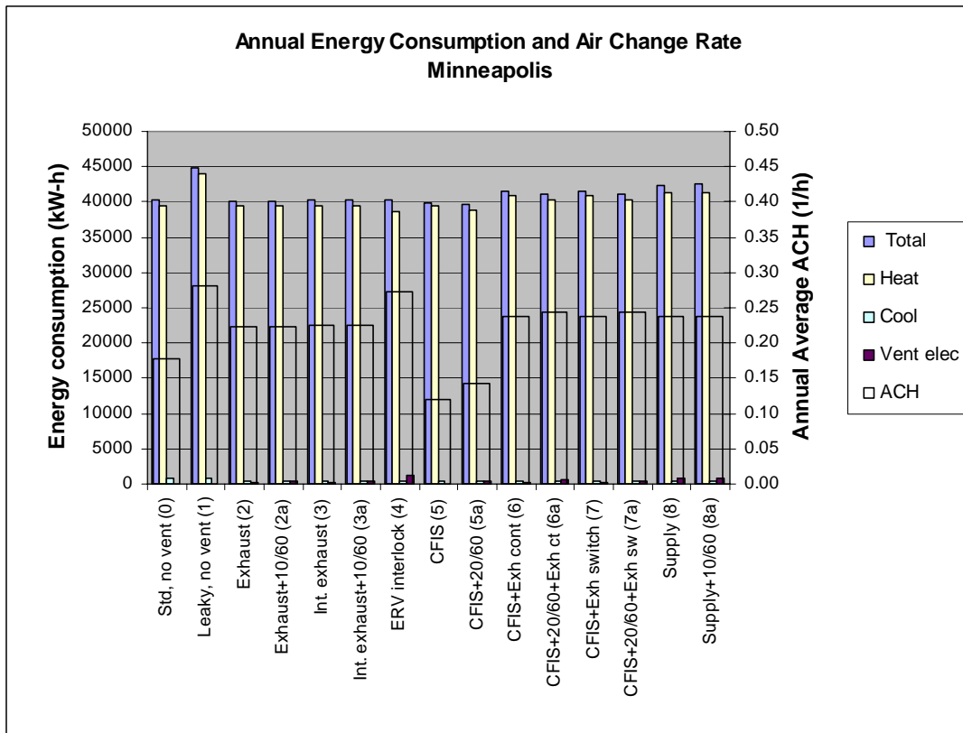
Figure B.12 Annual energy consumption and annual average air change rate for Minneapolis
