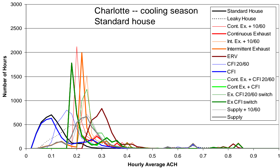
Figure A.33 Frequency distribution of hourly average air change rate (0.02 ach bins) for the cooling season in Charlotte
