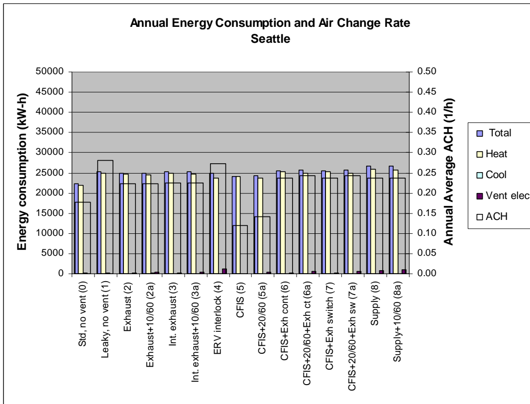
Figure B.10 Annual energy consumption and annual average air change rate for Seattle
