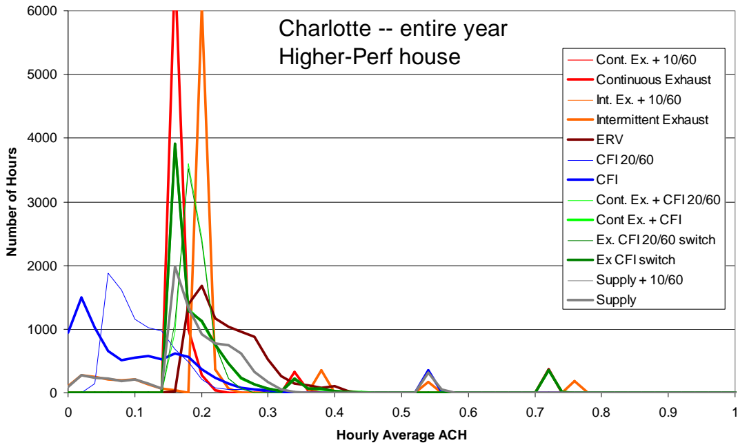
Figure B.32 Frequency distribution of hourly average air change rate (0.02 ach bins) for the entire year in Charlotte
