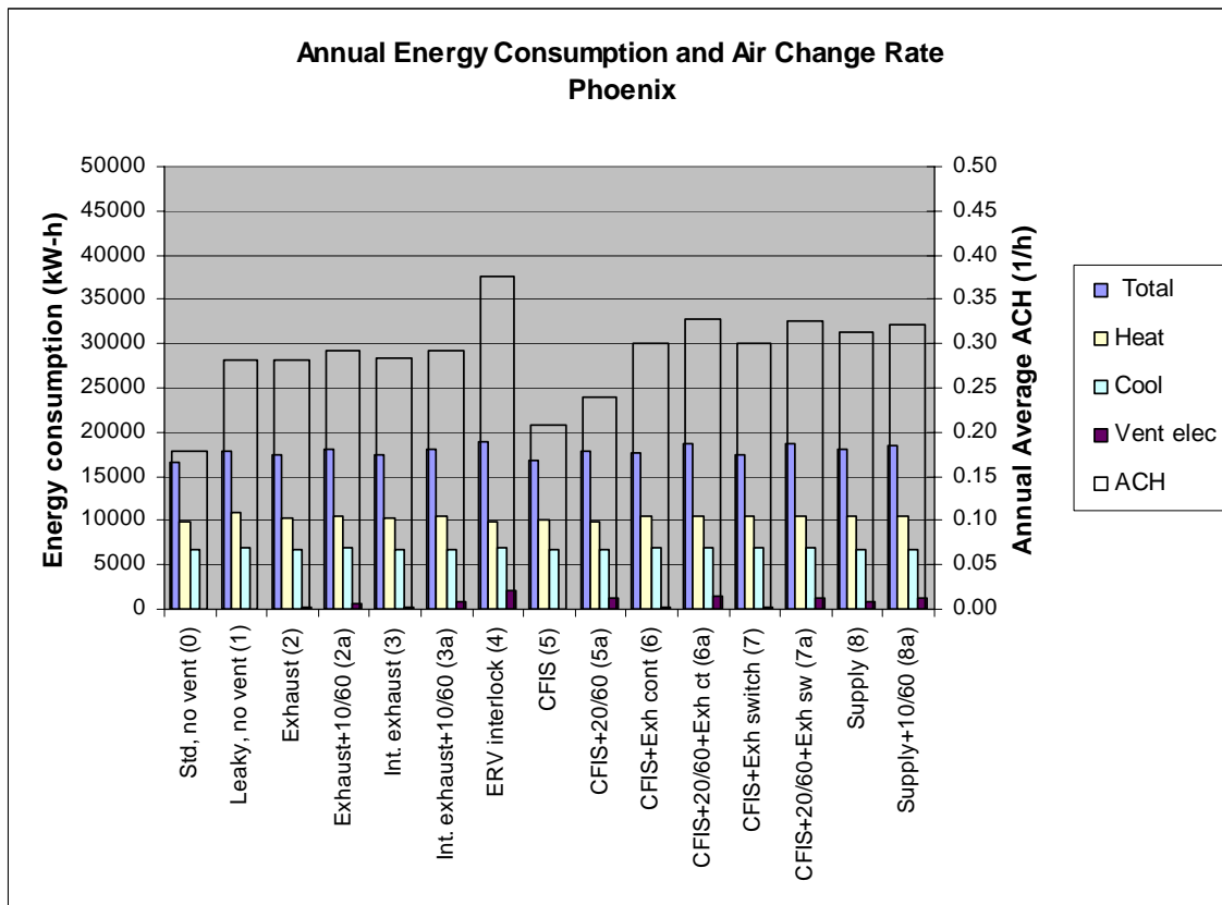
Figure A.4 Annual energy consumption and annual average air change rate for Phoenix
