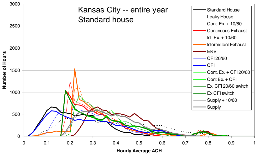
Figure A.35 Frequency distribution of hourly average air change rate (0.02 ach bins) for the entire year in Kansas City
