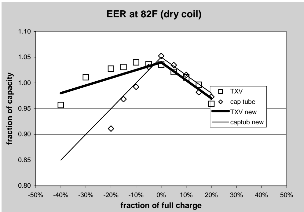
Figure C13. Dry Coil EER variation with charge
