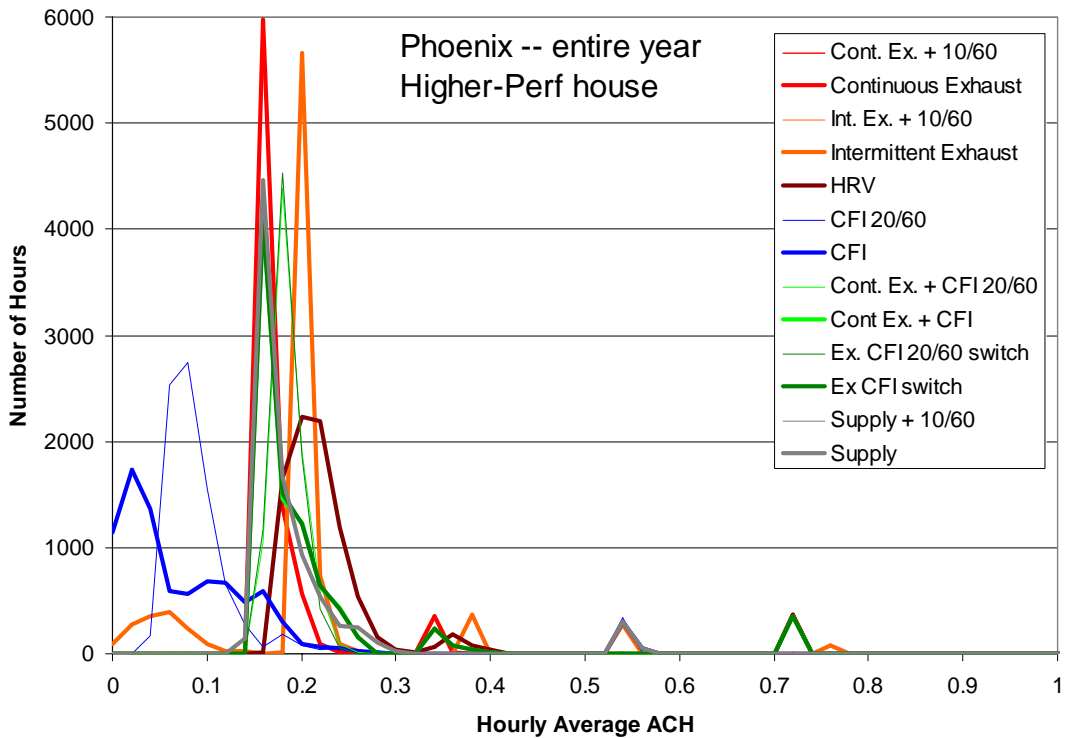
Figure 3.3(b) Hourly average air change rate (ach frequency in 0.02 bins) for Phoenix, for Higher-Performance house
