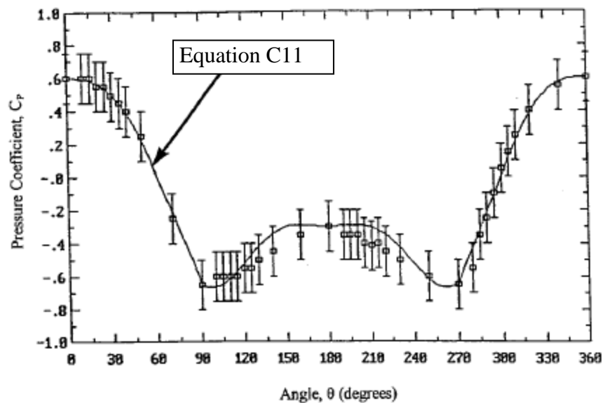
Figure C3. Angular variation in wind pressure coefficient for a rectangular building
