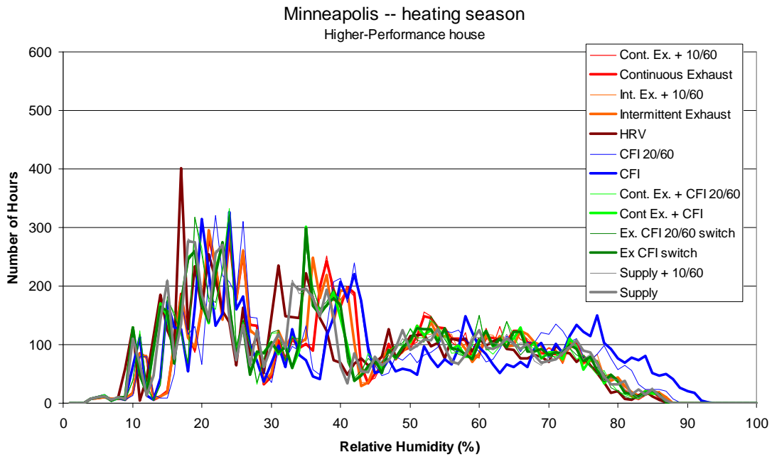
Figure B.26 Frequency distribution of hourly average indoor relative humidity (1% bins) for the heating season in Minneapolis
