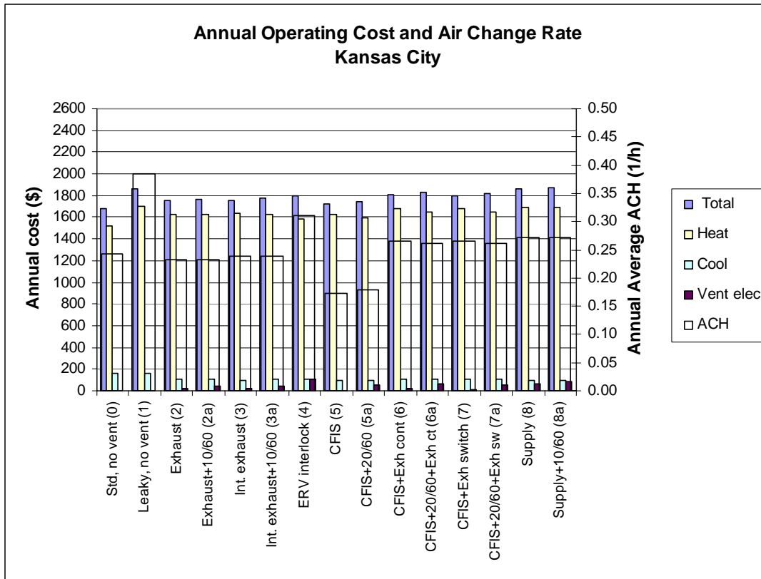
Figure B.7 Annual operating cost and annual average air change rate for Kansas City
