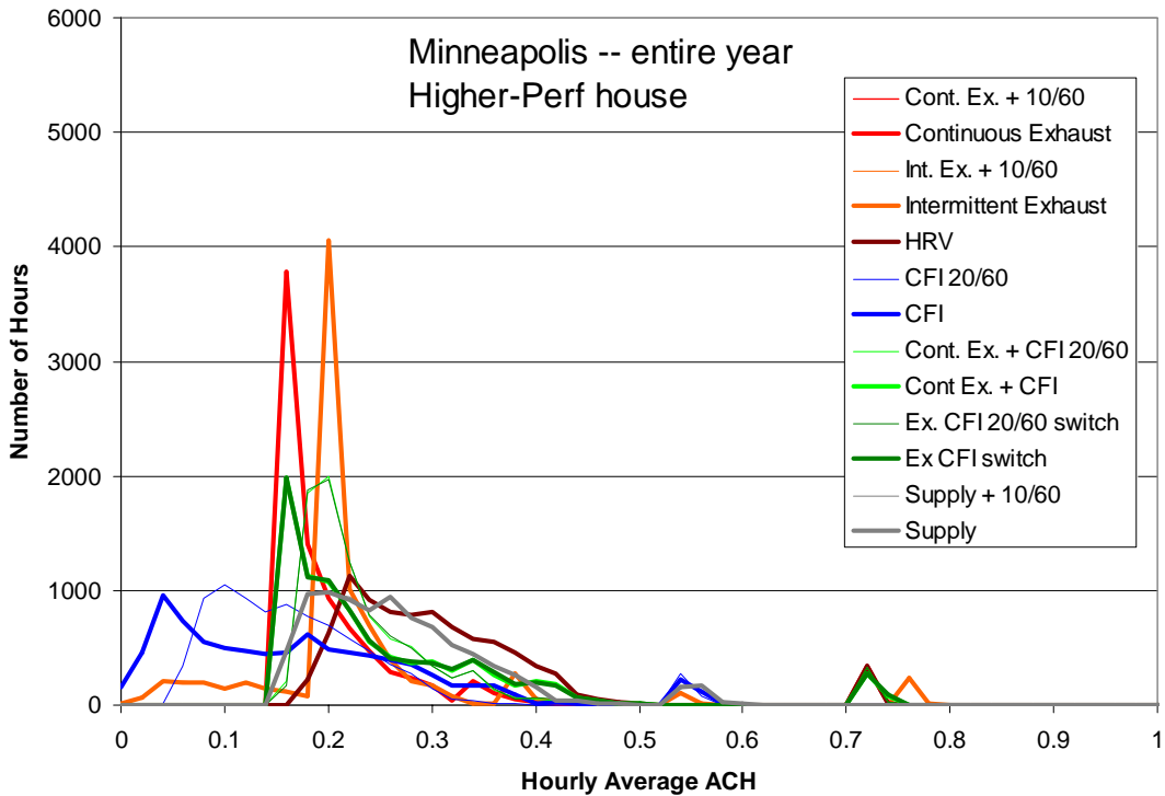
Figure B.40 Frequency distribution of hourly average air change rate (0.02 ach bins) for the entire year in Minneapolis
