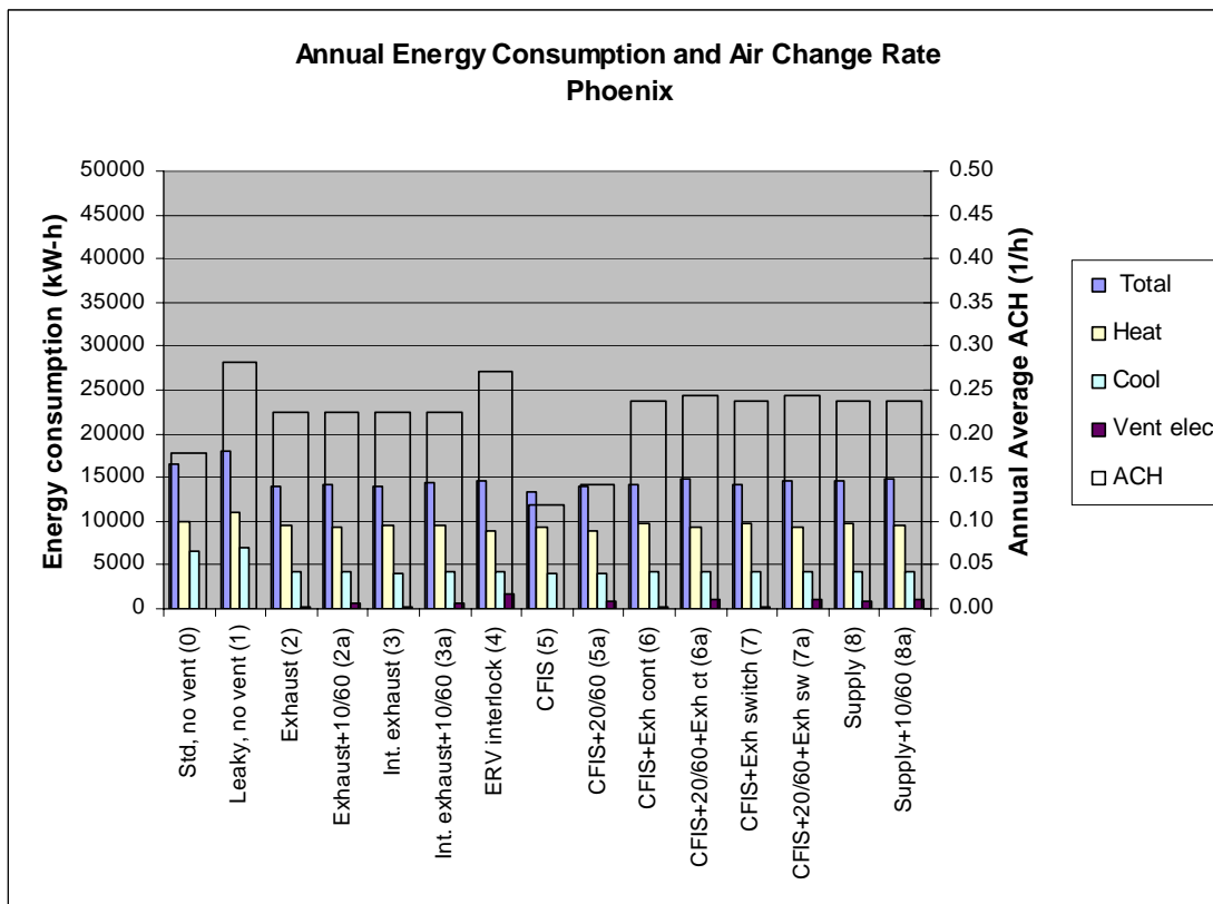
Figure B.4 Annual energy consumption and annual average air change rate for Phoenix
