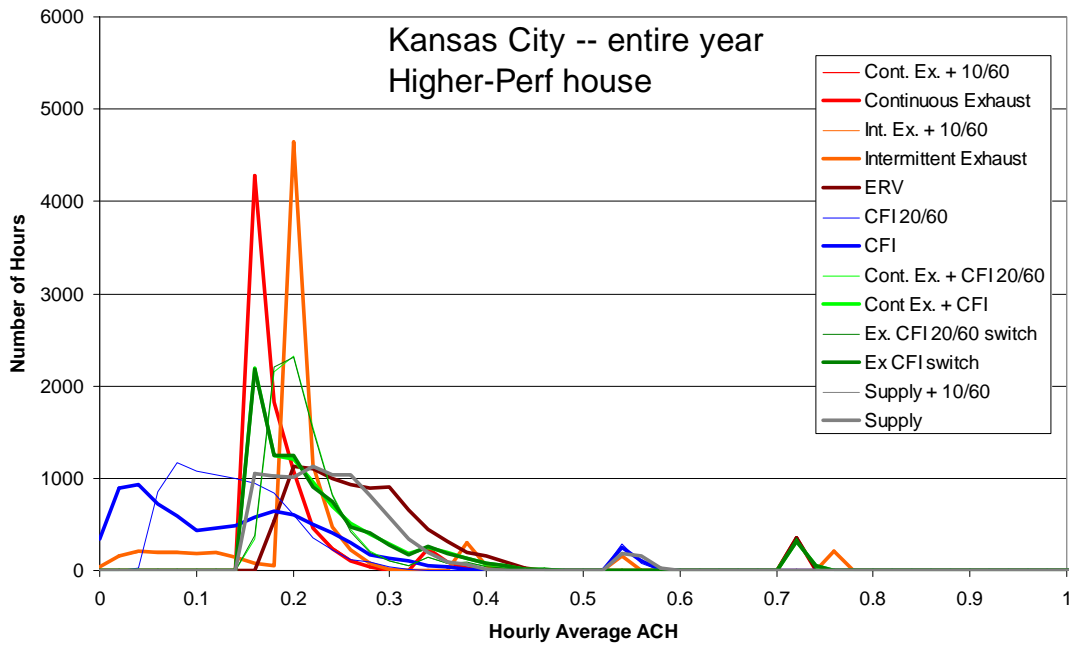
Figure B.35 Frequency distribution of hourly average air change rate (0.02 ach bins) for the entire year in Kansas City
