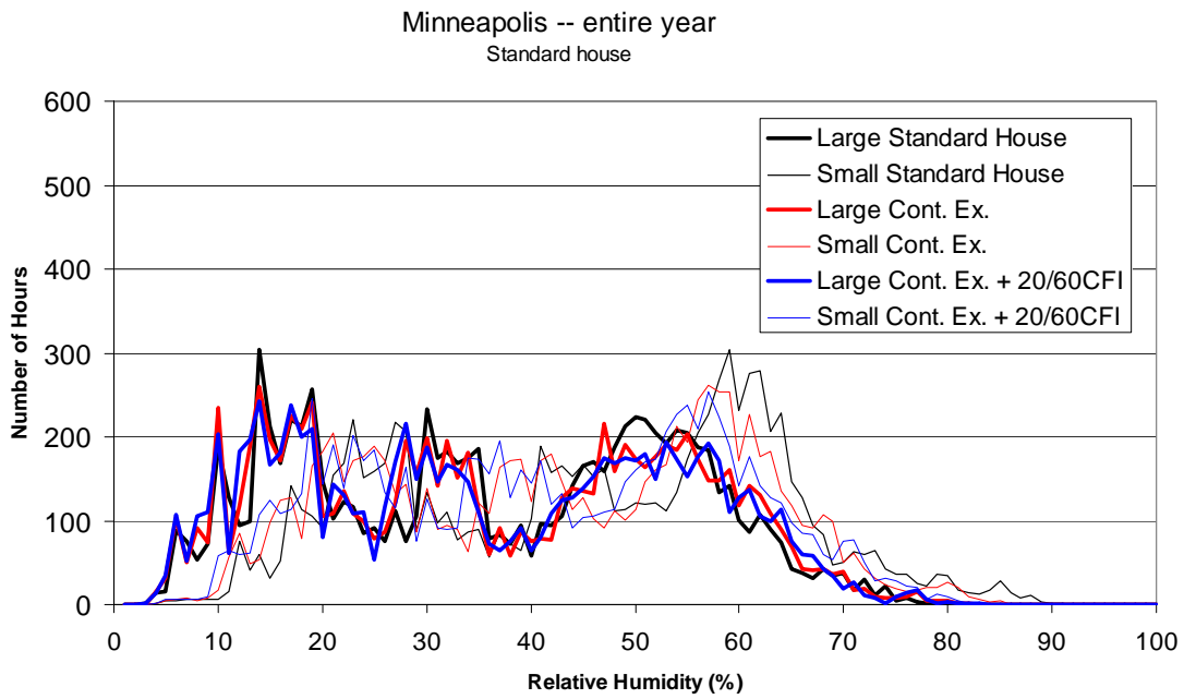
Figure 3.18 Frequency distribution of hourly average indoor relative humidity (1% bins) for large and small houses, for the Standard-Performance house in Minneapolis
