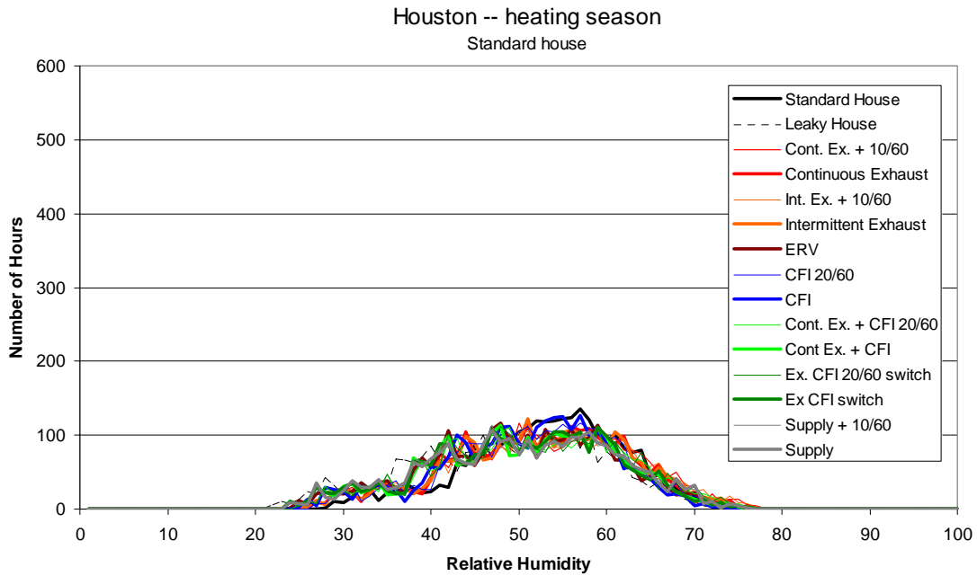
Figure 3.12(a) Frequency distribution of hourly average indoor relative humidity (1% RH bins) for the heating season for the Standard-Performance house in Houston
