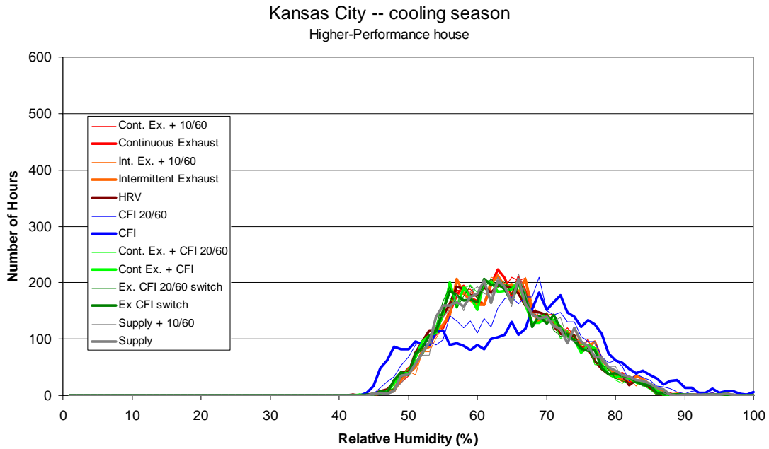
Figure B.20 Frequency distribution of hourly average indoor relative humidity (1% bins) for the cooling season in Kansas City
