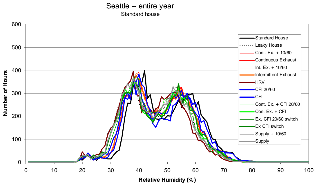
Figure A.22 Frequency distribution of hourly average indoor relative humidity (1% bins) for the entire year in Seattle
