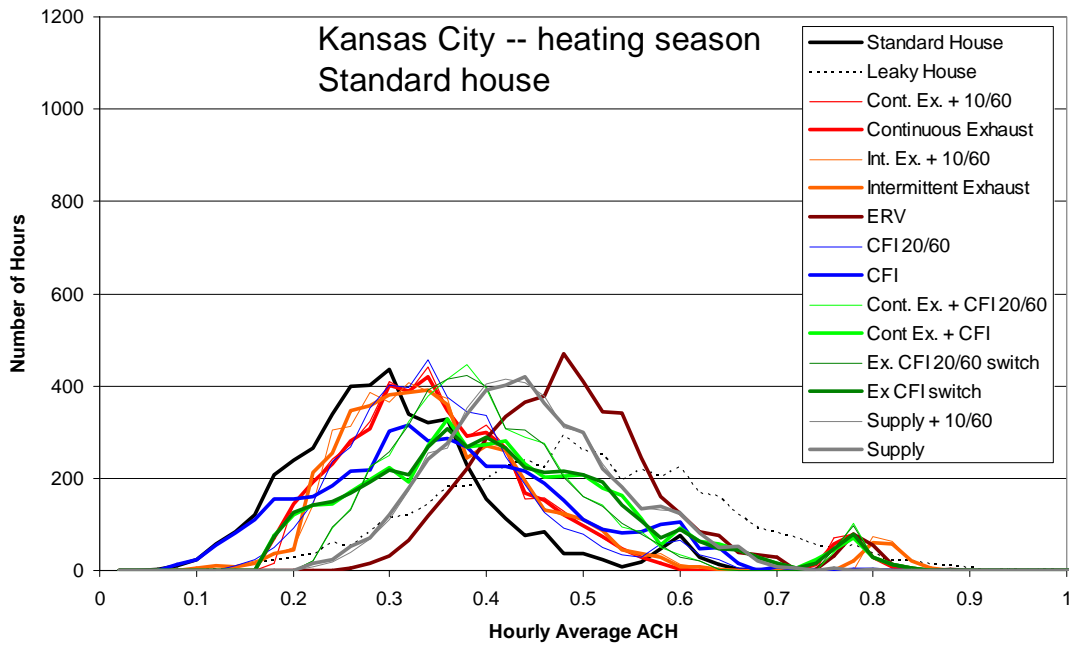
Figure A.37 Frequency distribution of hourly average air change rate (0.02 ach bins) for the heating season in Kansas City
