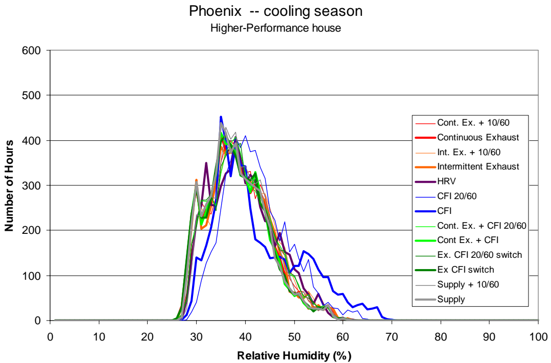
Figure B.14 Frequency distribution of hourly average indoor relative humidity (1% bins) for the cooling season in Phoenix
