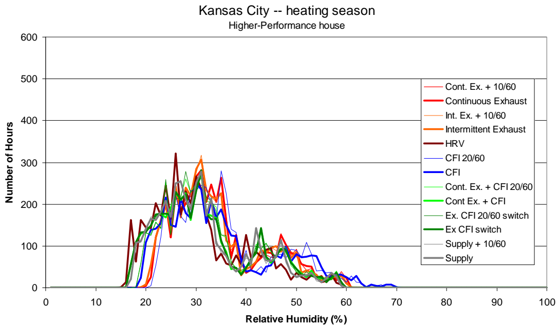
Figure B.21 Frequency distribution of hourly average indoor relative humidity (1% bins) for the heating season in Kansas City
