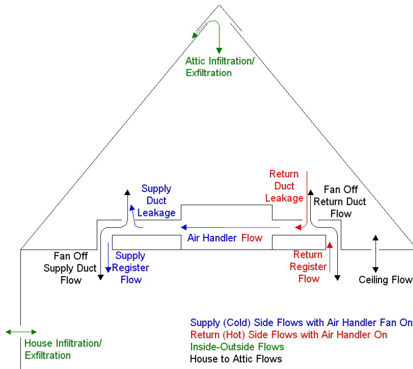
Figure C2: Schematic of duct related airflows (Arrows indicate direction). House and attic air infiltration/exfiltration is the sum of local and distributed leakage.
