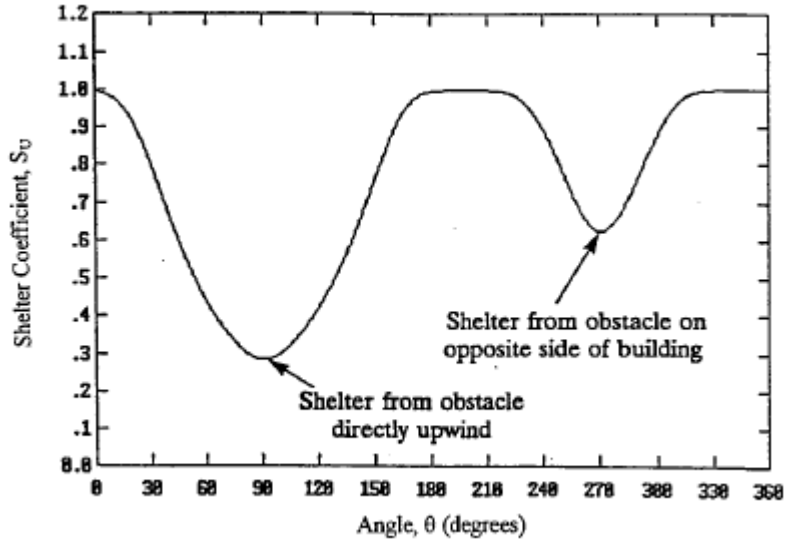
Figure C7. Wind shelter for a typical urban house
