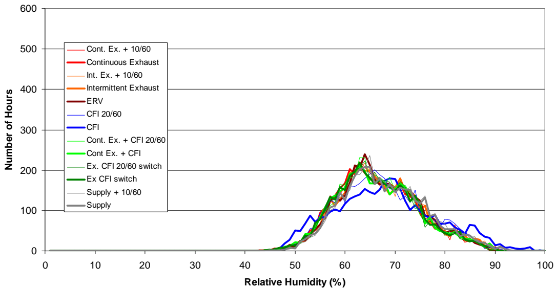
Figure B.17 Frequency distribution of hourly average indoor relative humidity (1% bins) for the cooling season in Charlotte
