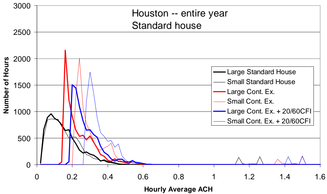
Figure 3.15 Frequency distribution of hourly average air change rate (0.02 ach bins) for large and small houses, for the Standard-Performance house in Houston
