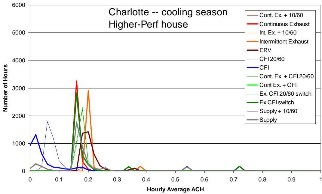
Figure B.33 Frequency distribution of hourly average air change rate (0.02 ach bins) for the cooling season in Charlotte
