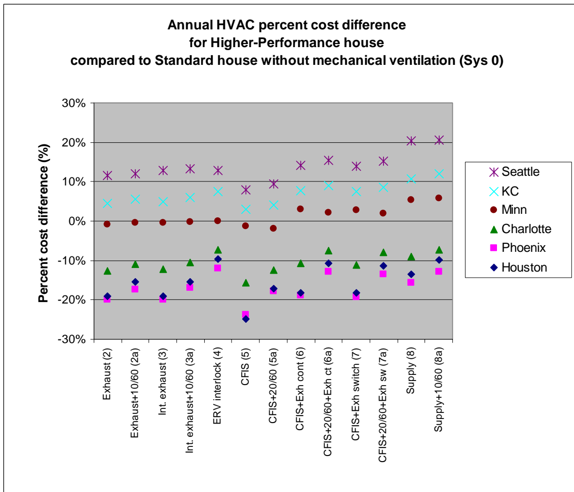
Figure 3.8(b) Annual HVAC percent cost difference for the Higher Performance house compared to the Standard house without mechanical ventilation, for all six climate locations
