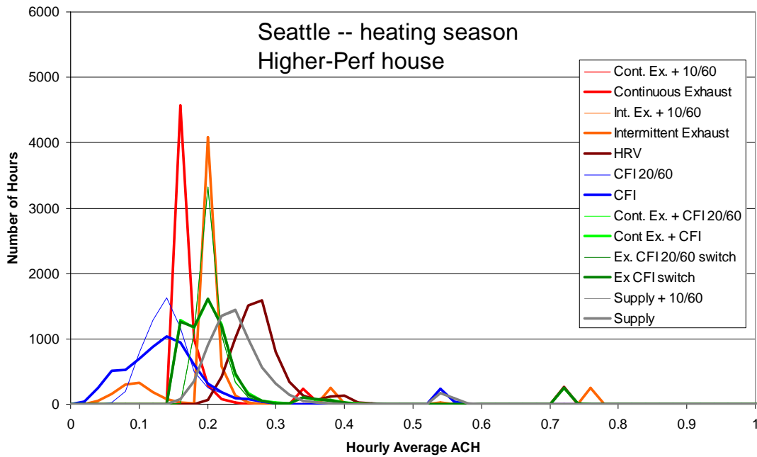
Figure B.39 Frequency distribution of hourly average air change rate (0.02 ach bins) for the heating season in Seattle
