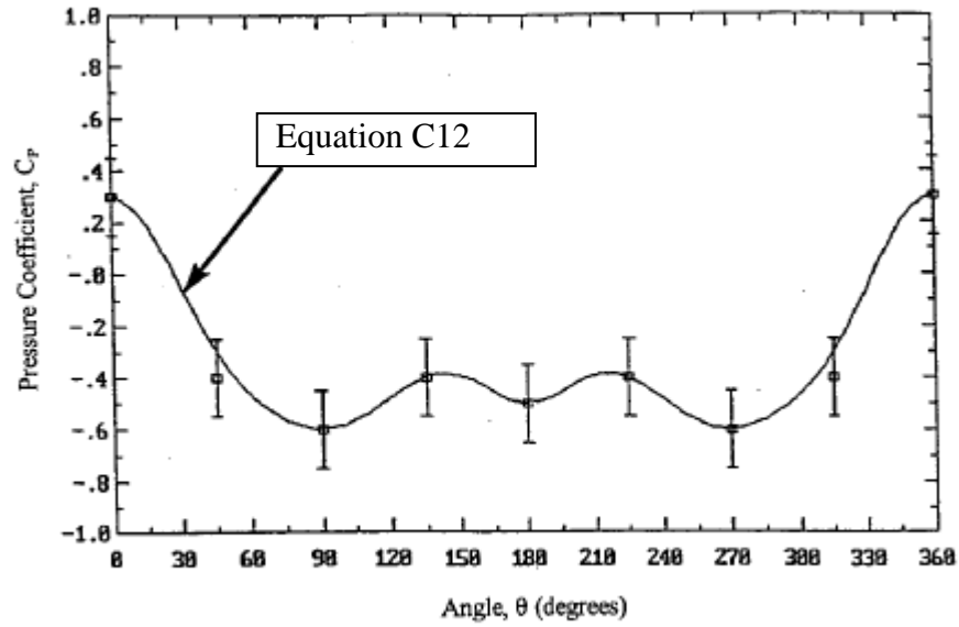
Figure C4. Roof pressure coefficients for a steep sloped roof (pitch > 30°)
