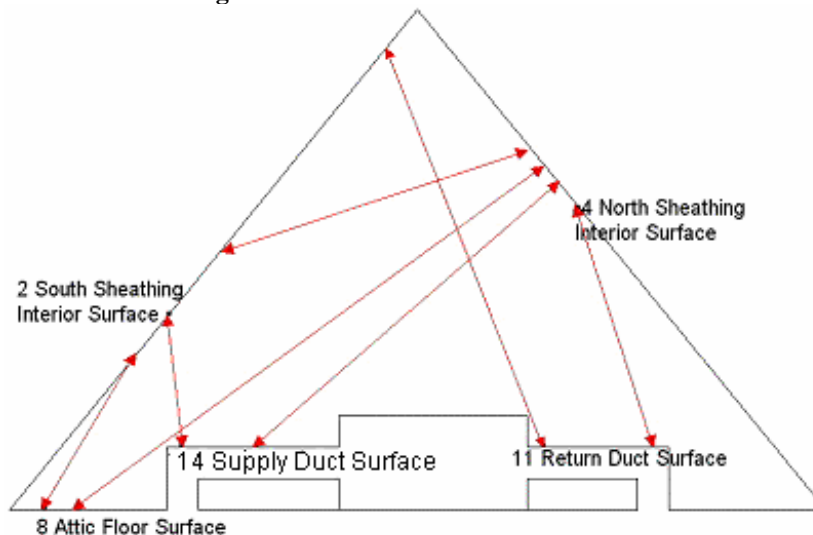
Figure C9: Radiation Transfer for Ducts in Attic
