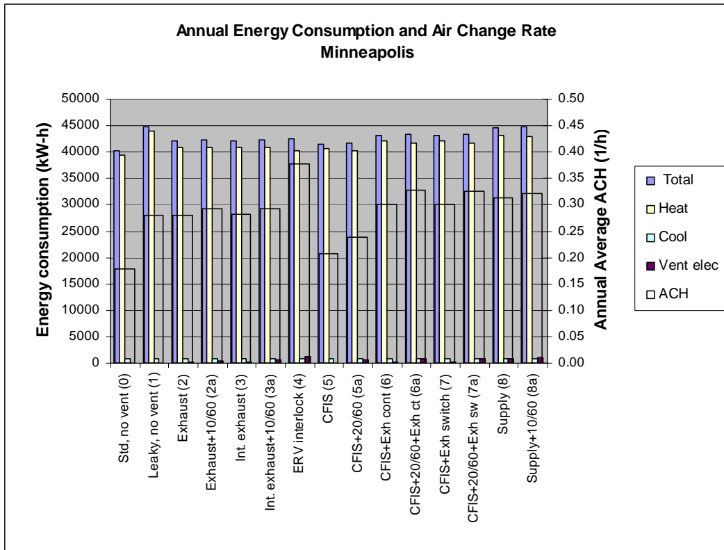
Figure A.12 Annual energy consumption and annual average air change rate for Minneapolis
