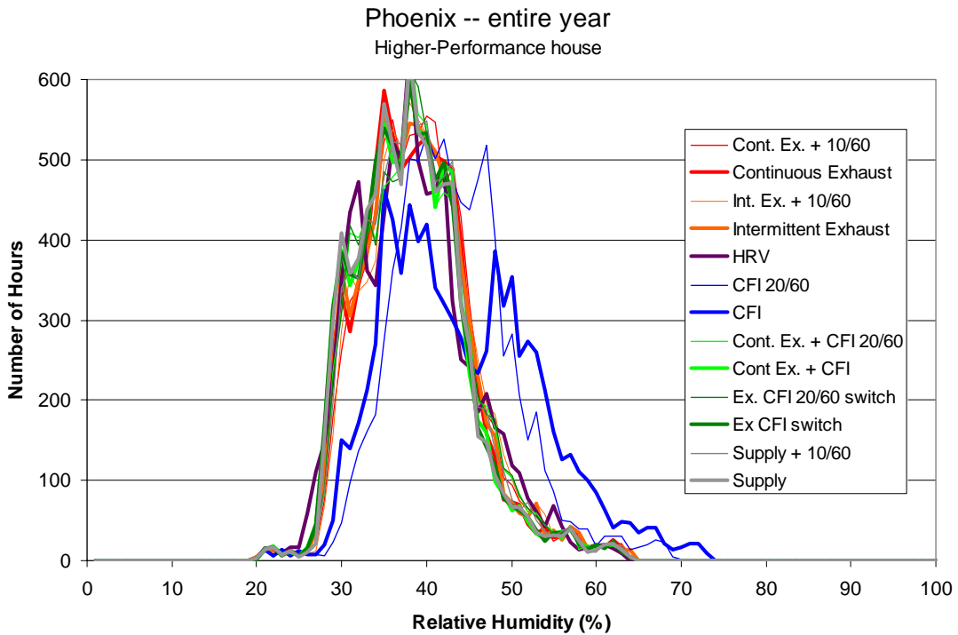
Figure B.13 Frequency distribution of hourly average indoor relative humidity (1% bins) for the entire year in Phoenix
