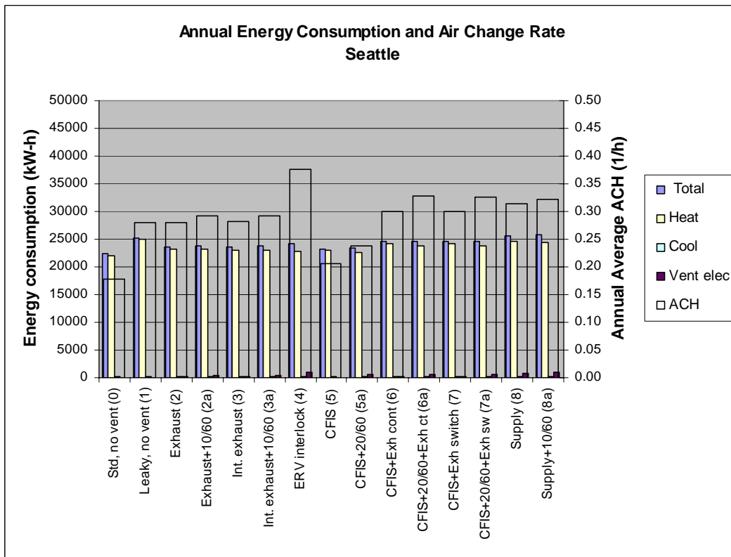
Figure A.10 Annual energy consumption and annual average air change rate for Seattle
