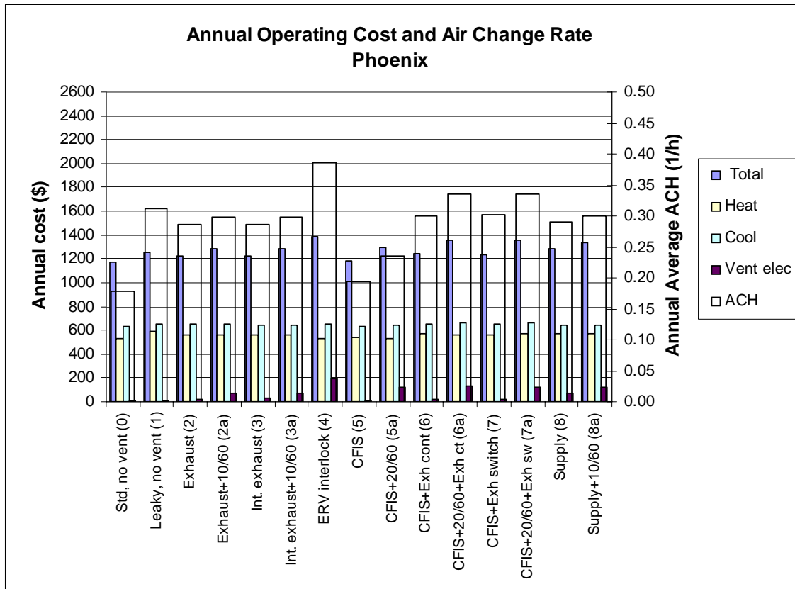
Figure A.3 Annual operating cost and annual average air change rate for Phoenix
