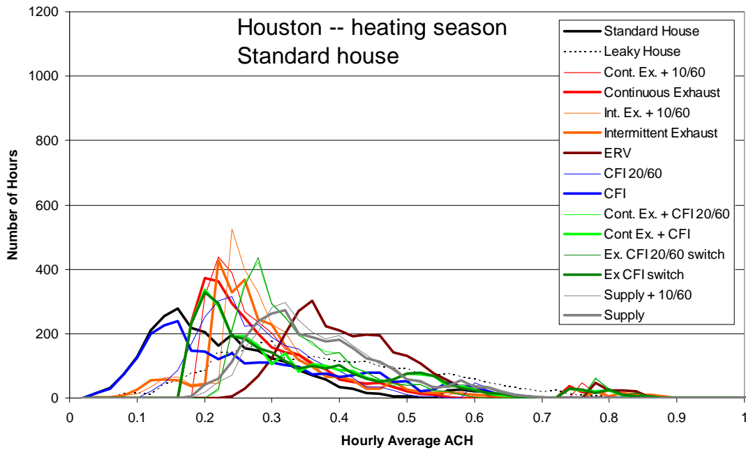
Figure A.29 Frequency distribution of hourly average air change rate (0.02 ach bins) for the heating season in Houston
