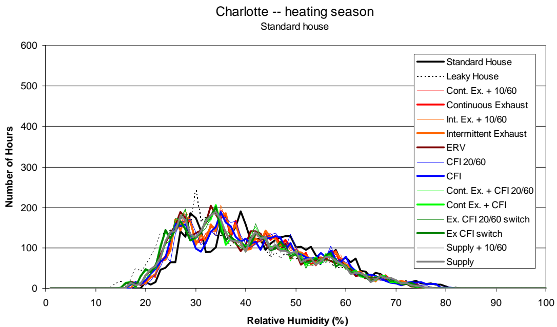
Figure A.18 Frequency distribution of hourly average indoor relative humidity (1% bins) for the heating season in Charlotte
