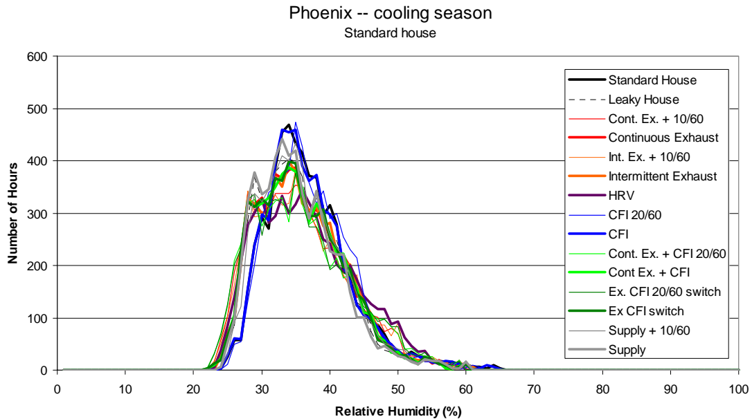
Figure A.14 Frequency distribution of hourly average indoor relative humidity (1% bins) for the cooling season in Phoenix
