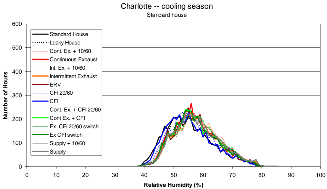
Figure A.17 Frequency distribution of hourly average indoor relative humidity (1% bins) for the cooling season in Charlotte
