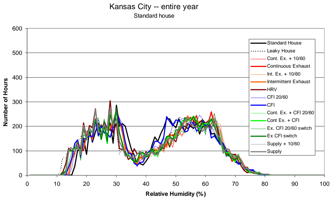
Figure A.19 Frequency distribution of hourly average indoor relative humidity (1% bins) for the entire year in Kansas City
