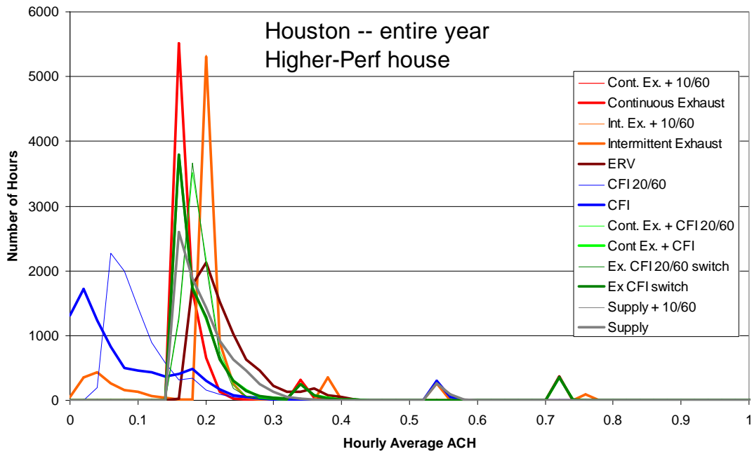
Figure B.27 Frequency distribution of hourly average air change rate (0.02 ach bins) for the entire year in Houston
