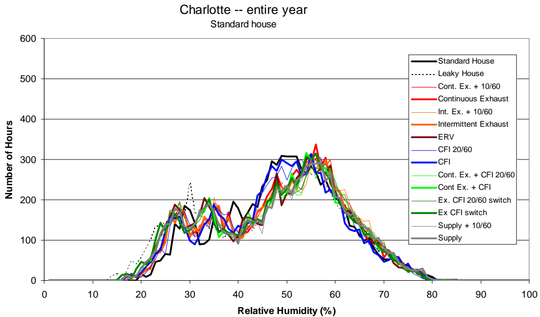
Figure A.16 Frequency distribution of hourly average indoor relative humidity (1% bins) for the entire year in Charlotte
