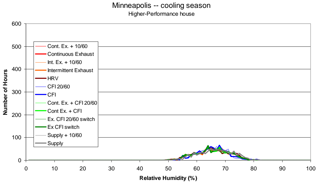
Figure B.25 Frequency distribution of hourly average indoor relative humidity (1% bins) for the cooling season in Minneapolis
