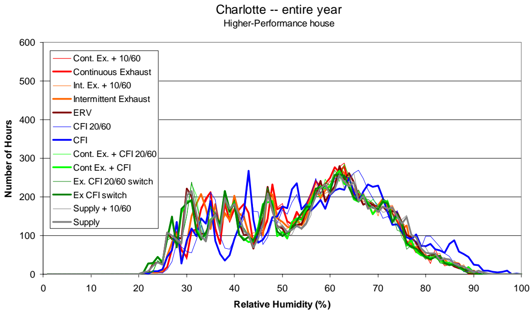
Figure B.16 Frequency distribution of hourly average indoor relative humidity (1% bins) for the entire year in Charlotte
