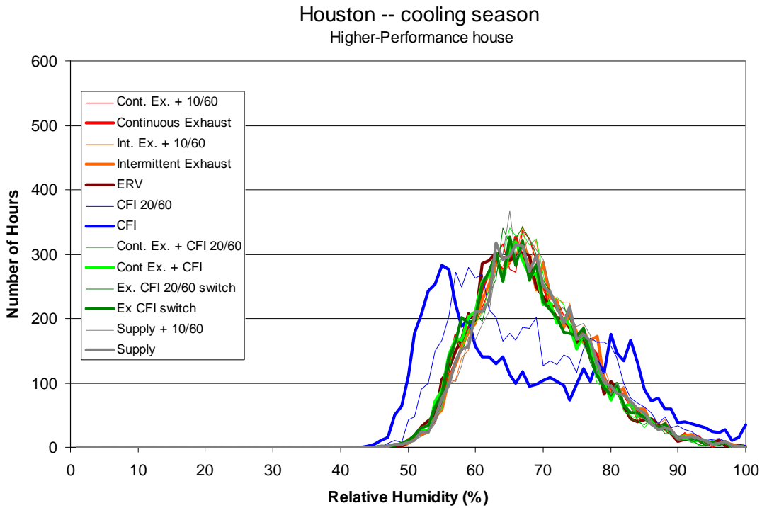
Figure 3.11(b) Frequency distribution of hourly average indoor relative humidity (1% RH bins) for the cooling season for the Higher-Performance house in Houston
