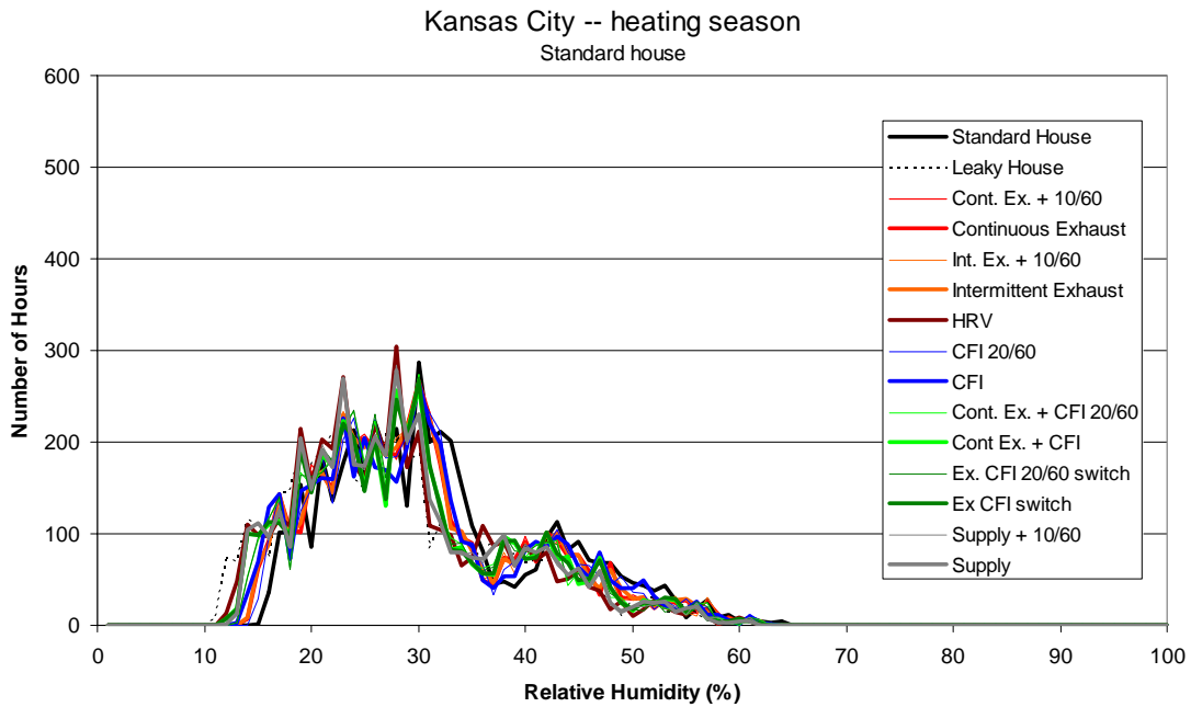
Figure A.21 Frequency distribution of hourly average indoor relative humidity (1% bins) for the heating season in Kansas City
