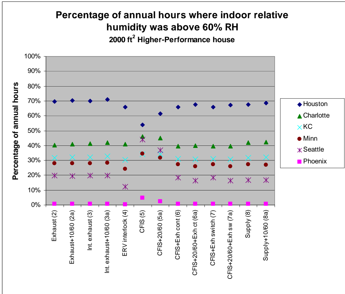
Figure 3.14(b) Percentage of annual hours where indoor relative humidity exceeded 60% RH for Higher-Performance house
