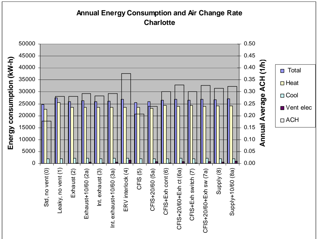
Figure A.6 Annual energy consumption and annual average air change rate for Charlotte
