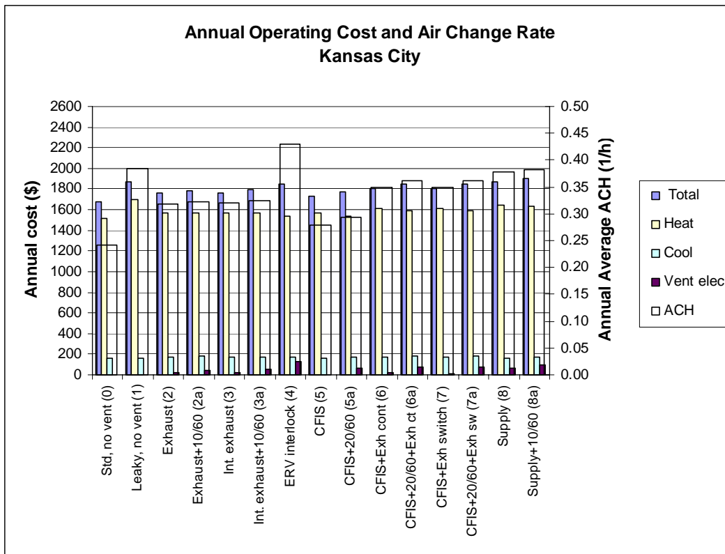
Figure A.7 Annual operating cost and annual average air change rate for Kansas City
