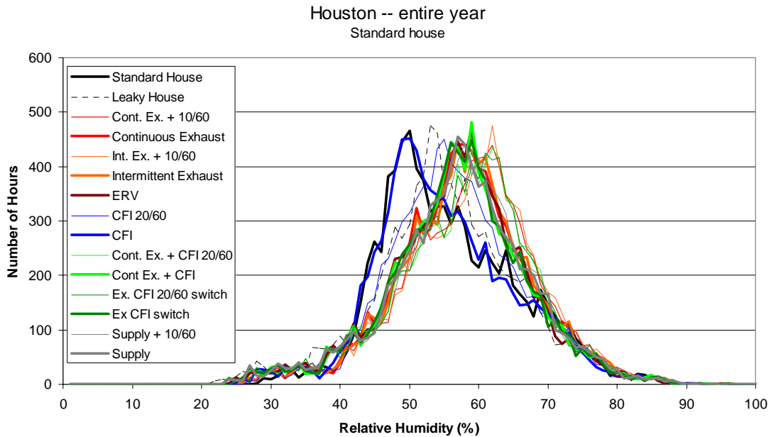
Figure 3.10(a) Frequency distribution of hourly average indoor relative humidity (1% RH bins) for the entire year for the Standard-Performance house in Houston
