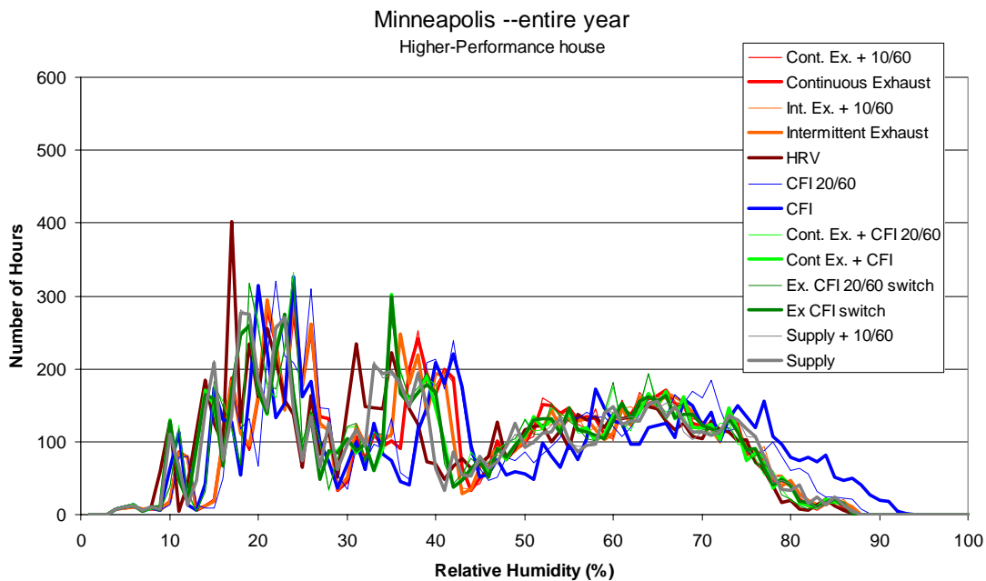
Figure 3.13(b) Frequency distribution of hourly average indoor relative humidity (1% RH bins) for the entire year for the Higher-Performance house in Minneapolis
