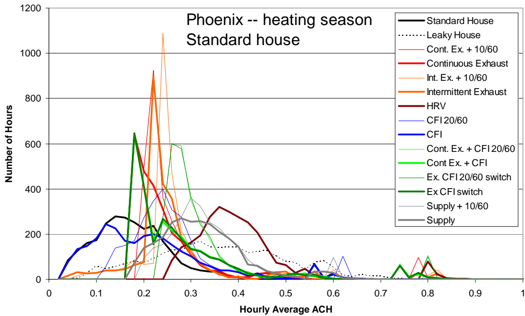
Figure A.31 Frequency distribution of hourly average air change rate (0.02 ach bins) for the heating season in Phoenix
