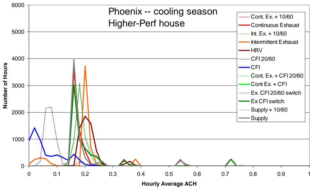
Figure B.30 Frequency distribution of hourly average air change rate (0.02 ach bins) for the cooling season in Phoenix
