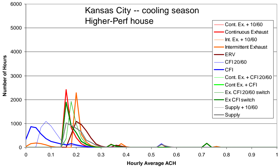
Figure B.36 Frequency distribution of hourly average air change rate (0.02 ach bins) for the cooling season in Kansas City
