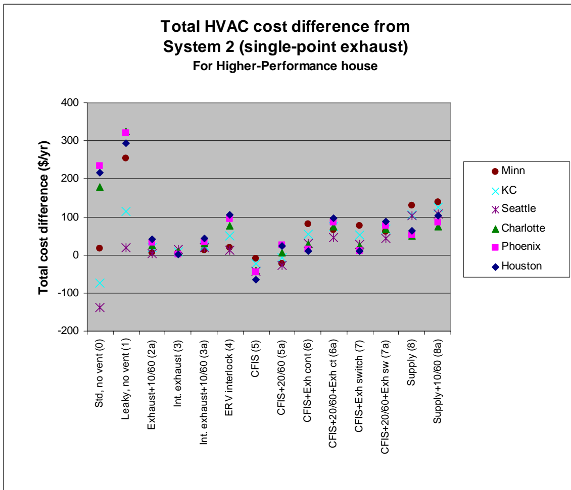
Figure 3.6(b) Total HVAC operating cost difference for the Higher-Performance house compared to System 2 (single-point exhaust), for all six climate locations
