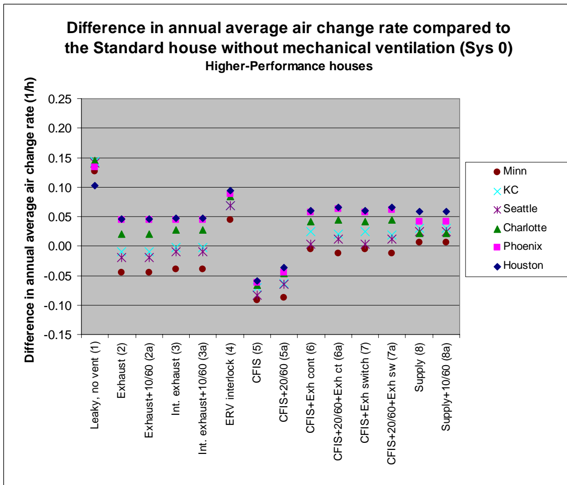
Figure 3.2(b) Difference in annual average air change rate (ach) for Higher-Performance houses (Systems 2 to 8a) compared to the Standard house without mechanical ventilation
