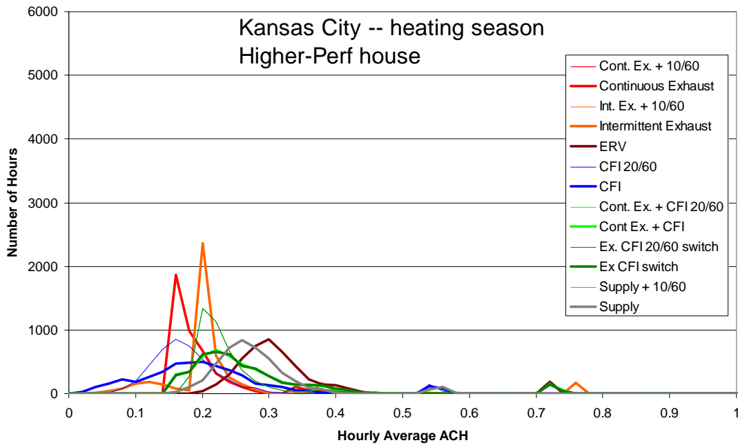
Figure B.37 Frequency distribution of hourly average air change rate (0.02 ach bins) for the heating season in Kansas City
