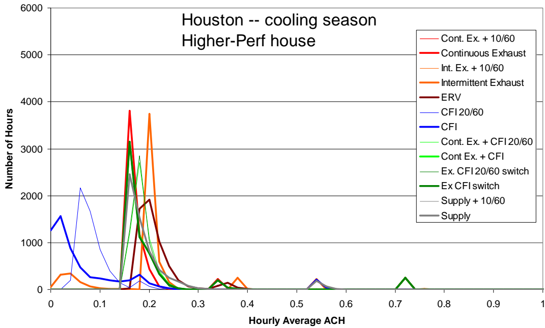
Figure B.28 Frequency distribution of hourly average air change rate (0.02 ach bins) for the cooling season in Houston
