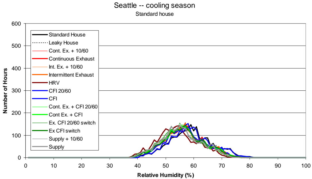
Figure A.23 Frequency distribution of hourly average indoor relative humidity (1% bins) for the cooling season in Seattle
