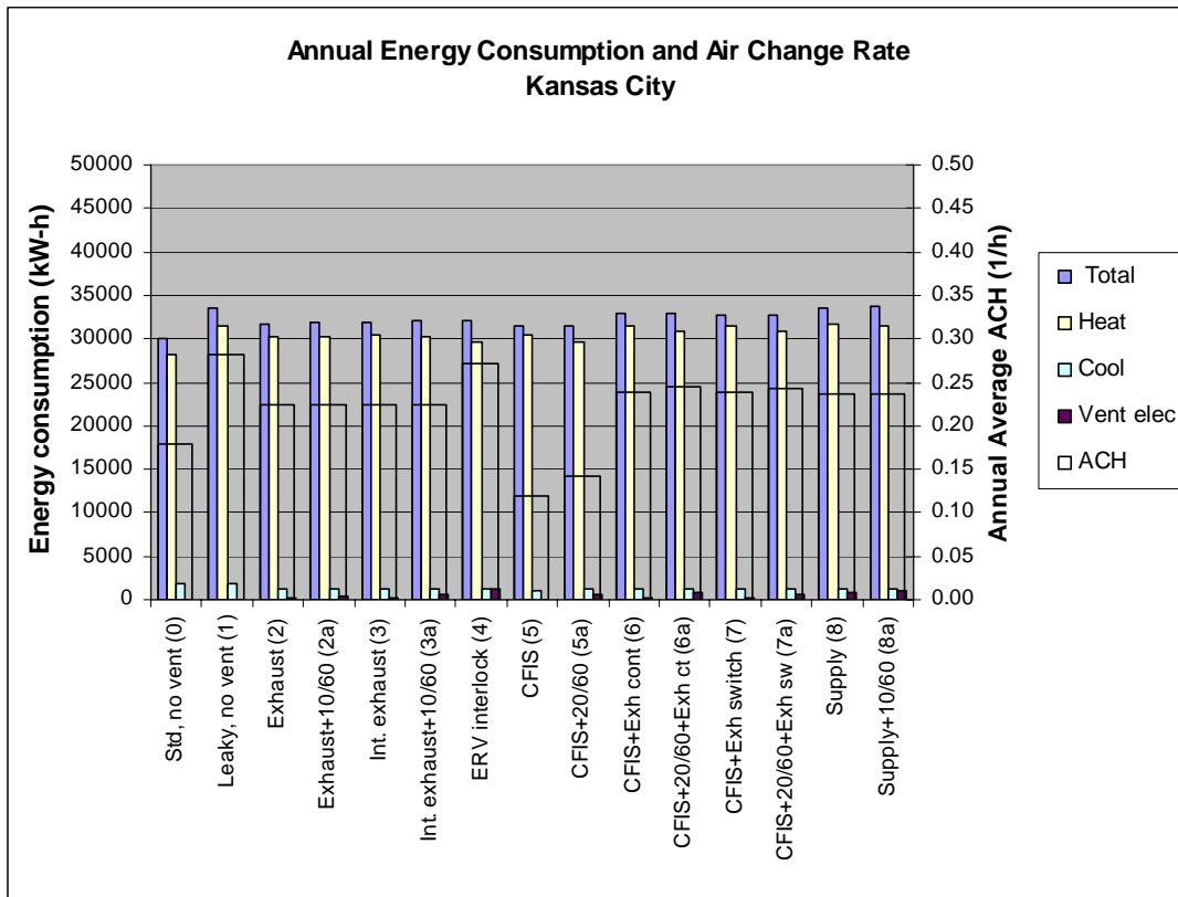
Figure B.8 Annual energy consumption and annual average air change rate for Kansas City
