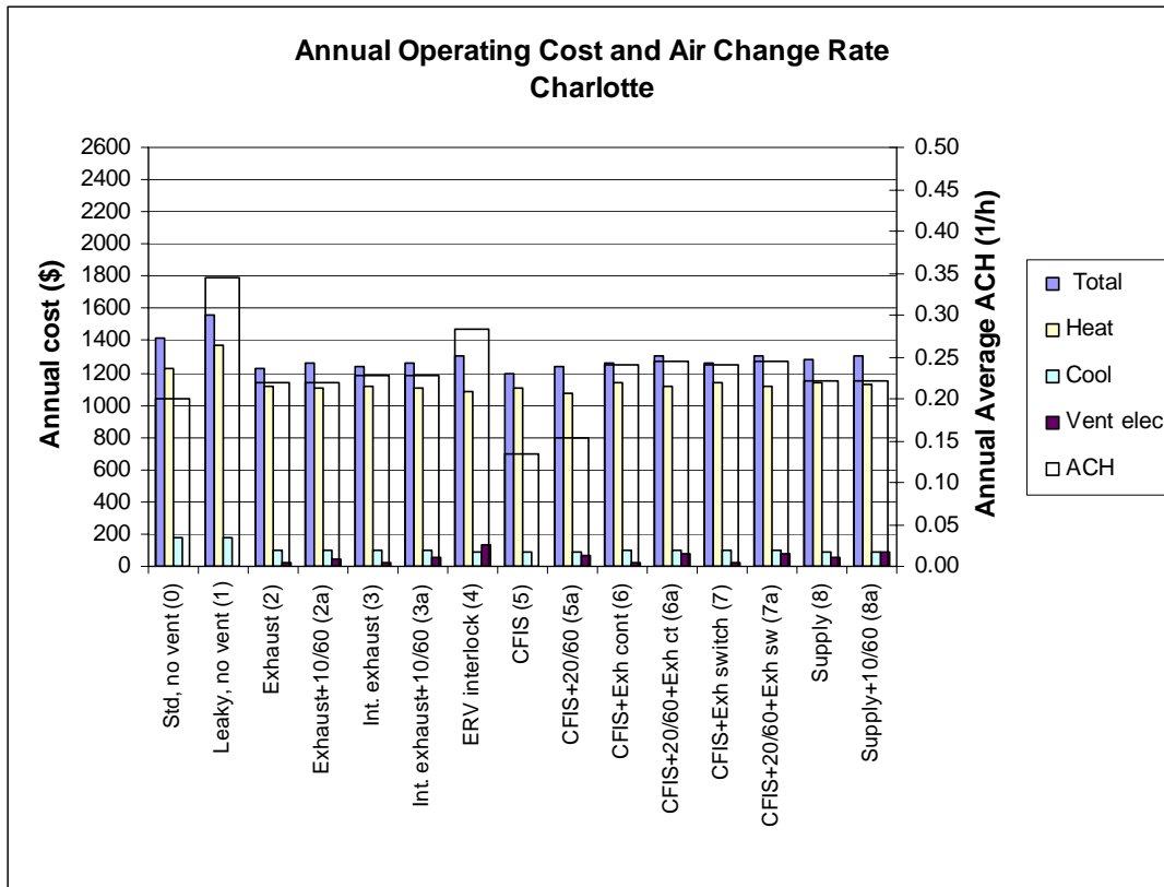
Figure B.5 Annual operating cost and annual average air change rate for Charlotte
