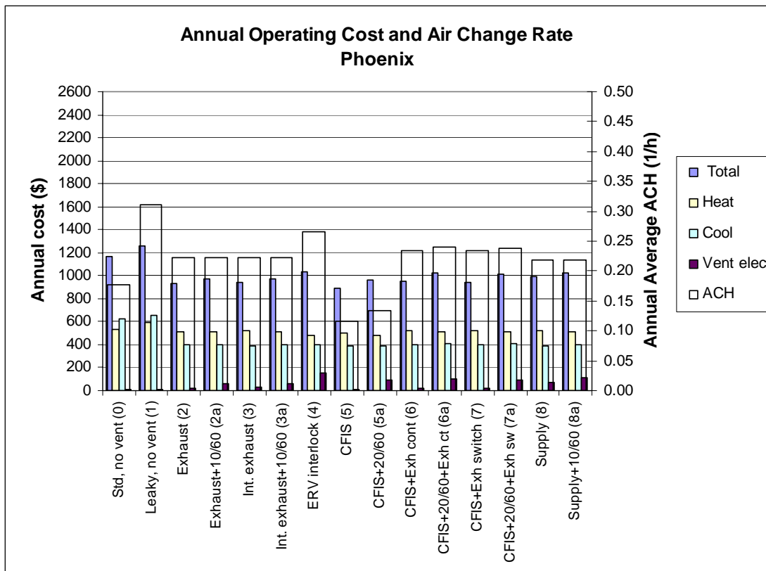
Figure B.3 Annual operating cost and annual average air change rate for Phoenix
