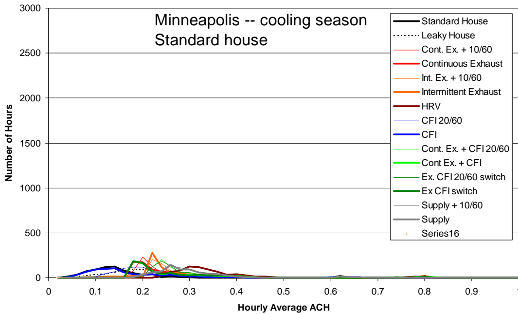
Figure A.41 Frequency distribution of hourly average air change rate (0.02 ach bins) for the cooling season in Minneapolis
