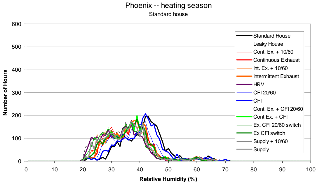
Figure A.15 Frequency distribution of hourly average indoor relative humidity (1% bins) for the heating season in Phoenix
