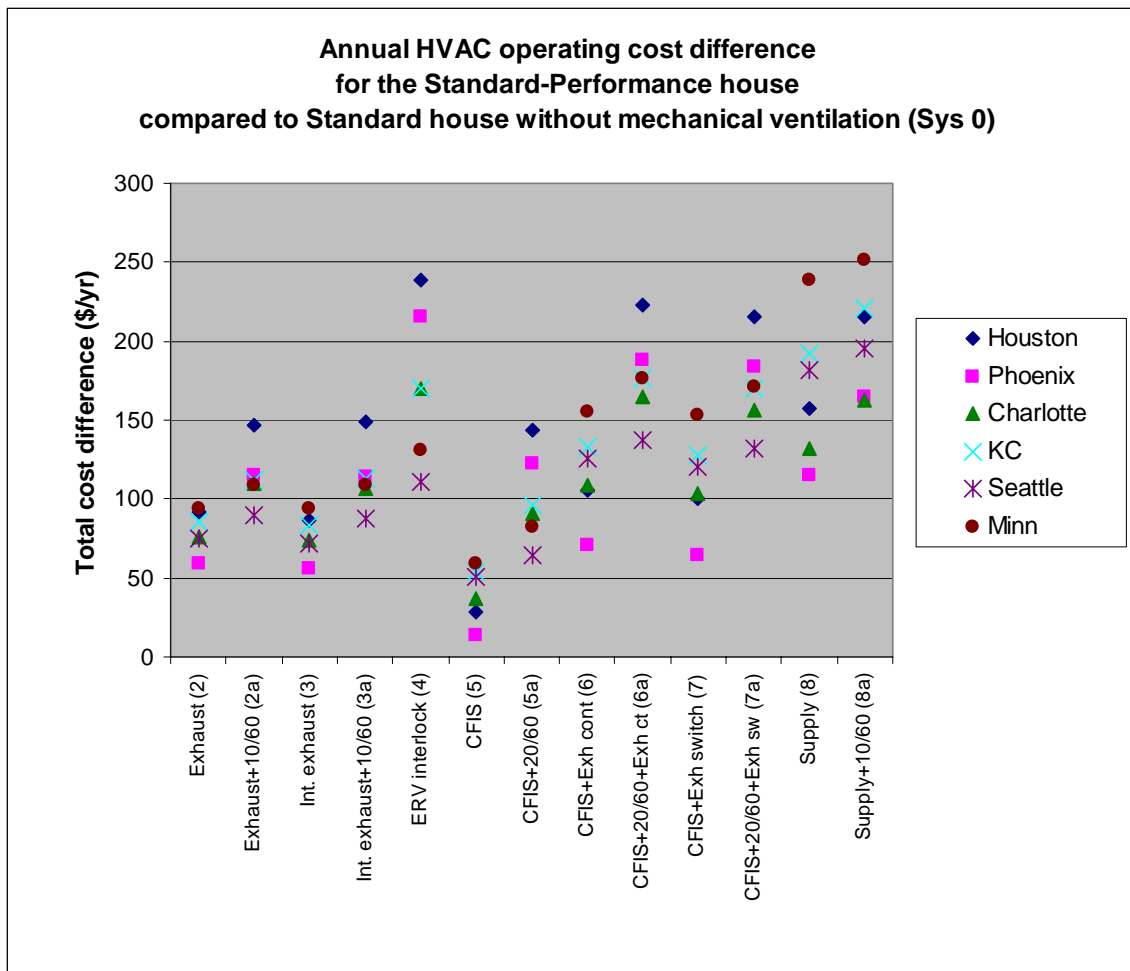
Figure 3.7(a) Annual HVAC operating cost difference compared to the Standard house without mechanical ventilation, for Standard-Performance houses in all six climate locations
