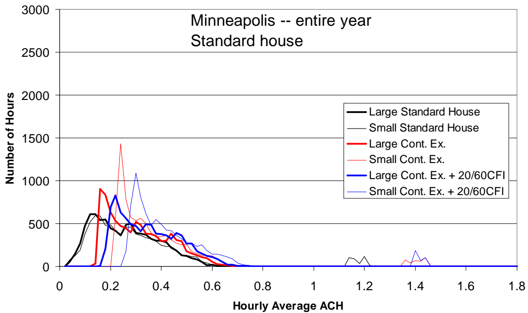
Figure 3.16 Frequency distribution of hourly average air change rate (0.02 ach bins) for large and small houses, for the Standard-Performance house in Minneapolis
