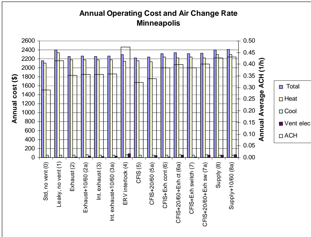
Figure A.11 Annual operating cost and annual average air change rate for Minneapolis
