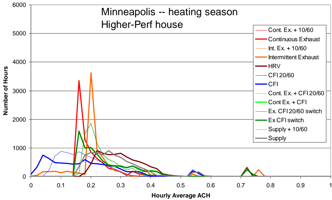
Figure B.42 Frequency distribution of hourly average air change rate (0.02 ach bins) for the heating season in Minneapolis
