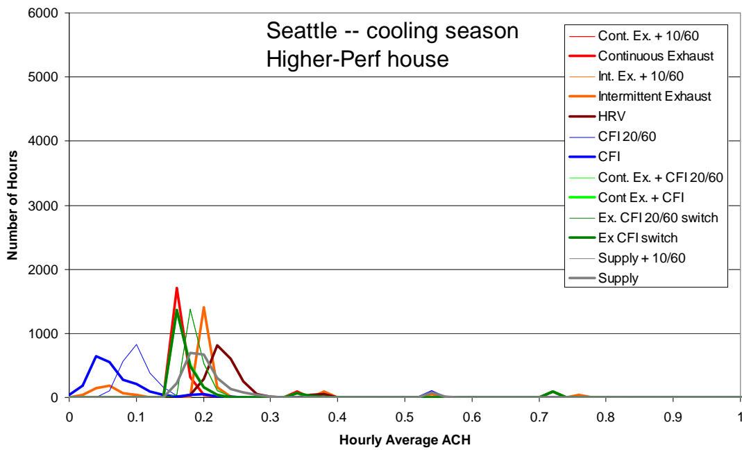
Figure B.38 Frequency distribution of hourly average air change rate (0.02 ach bins) for the cooling season in Seattle
