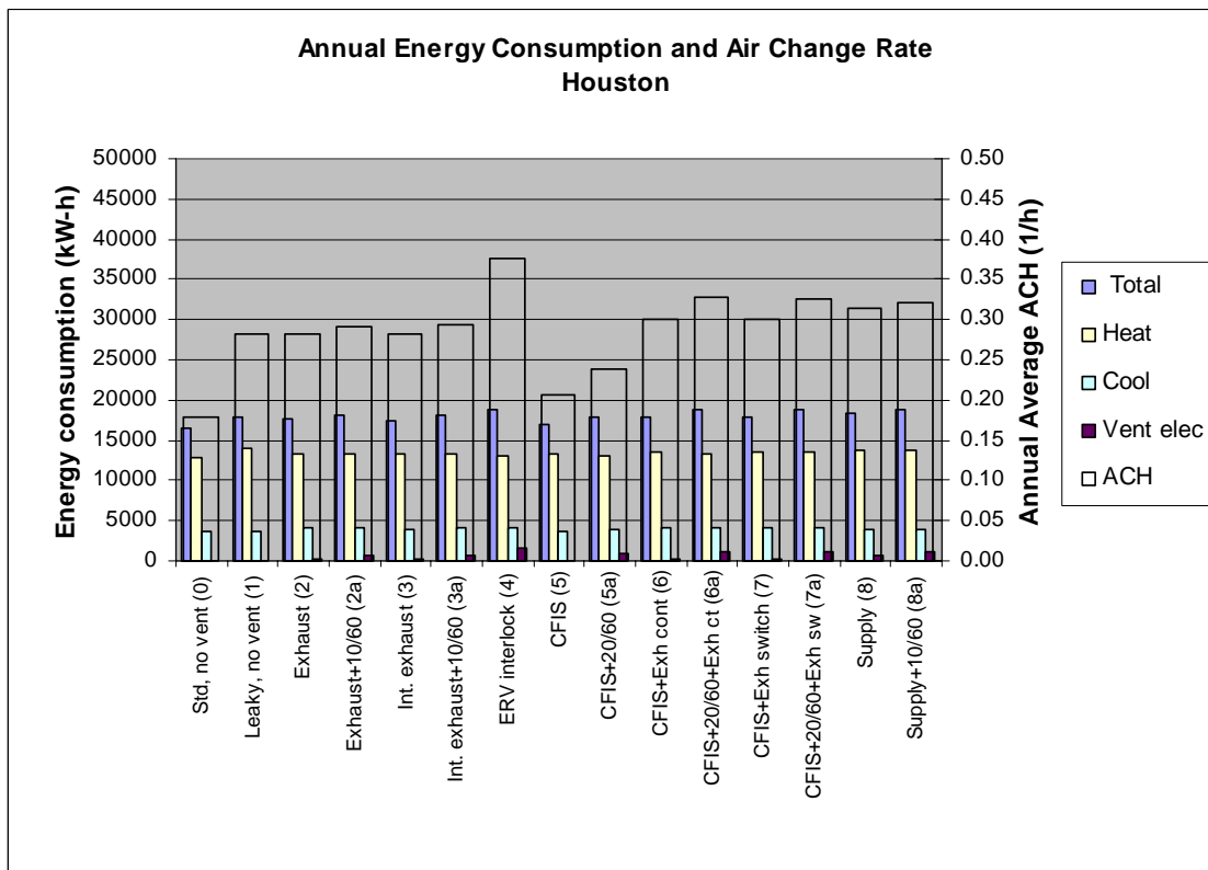
Figure A.2 Annual energy consumption and annual average air change rate for Houston
