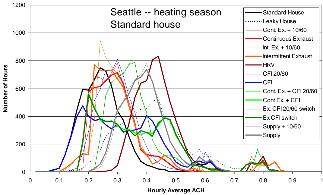
Figure A.39 Frequency distribution of hourly average air change rate (0.02 ach bins) for the heating season in Seattle
