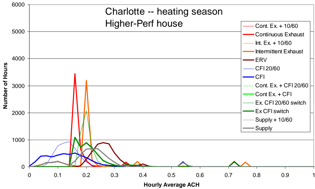
Figure B.34 Frequency distribution of hourly average air change rate (0.02 ach bins) for the heating season in Charlotte
