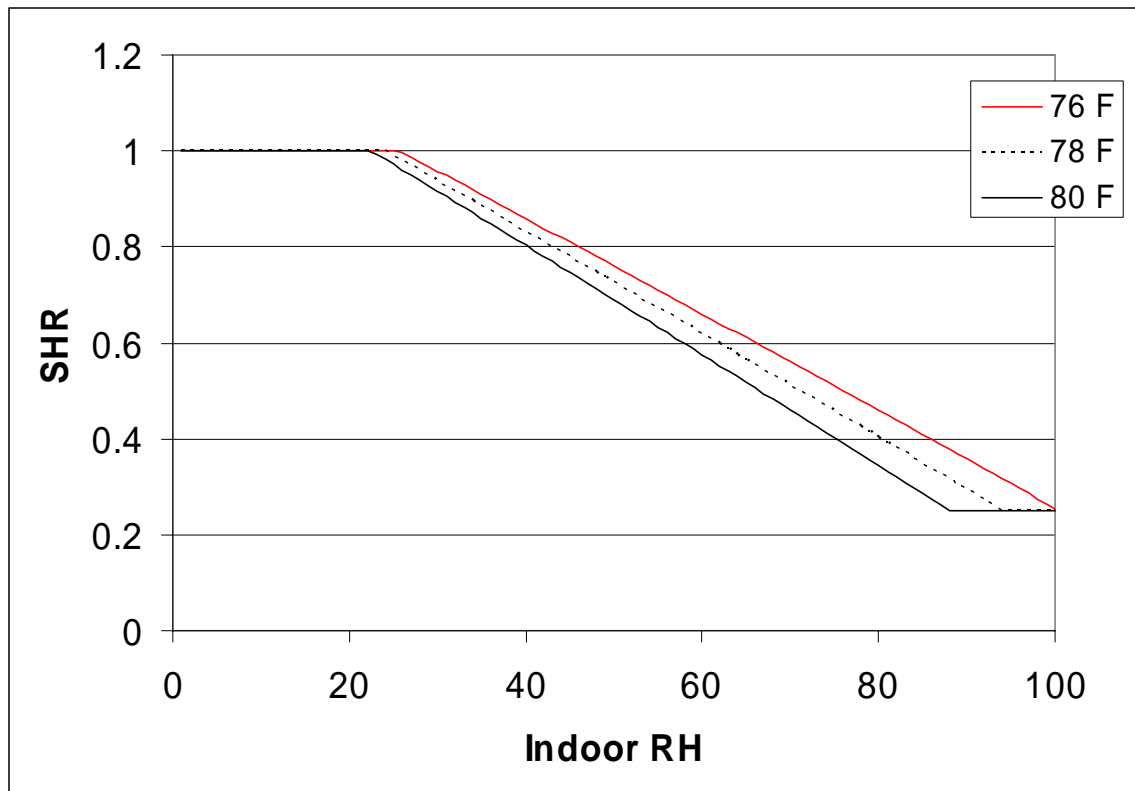
Figure 2.1 Illustration of SHR variability with indoor temperature and humidity
