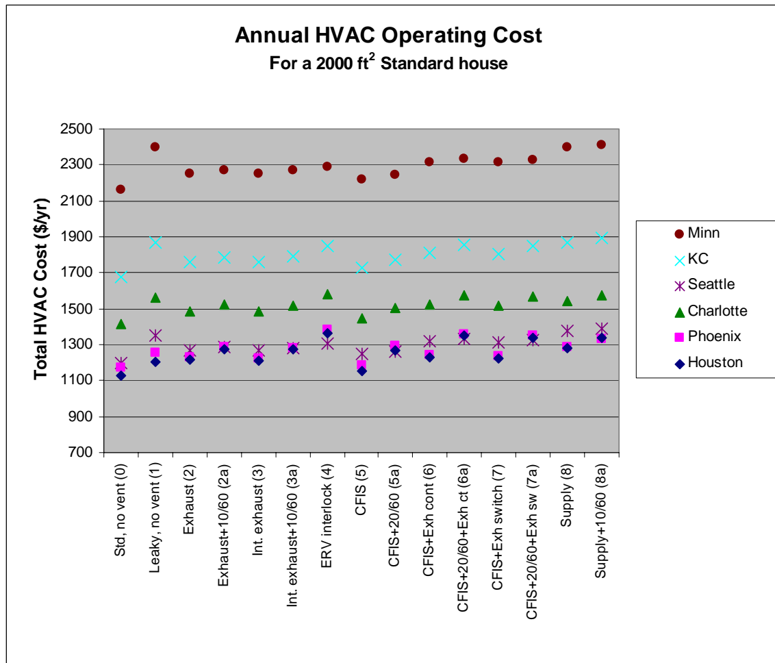
Figure 3.5(a) Comparison of annual HVAC operating cost (heating, cooling, and ventilation) for the Standard-Performance house, for all six climate locations
