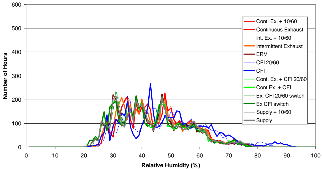
Figure B.18 Frequency distribution of hourly average indoor relative humidity (1% bins) for the heating season in Charlotte
