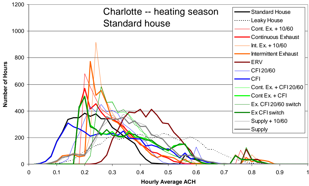
Figure A.34 Frequency distribution of hourly average air change rate (0.02 ach bins) for the heating season in Charlotte
