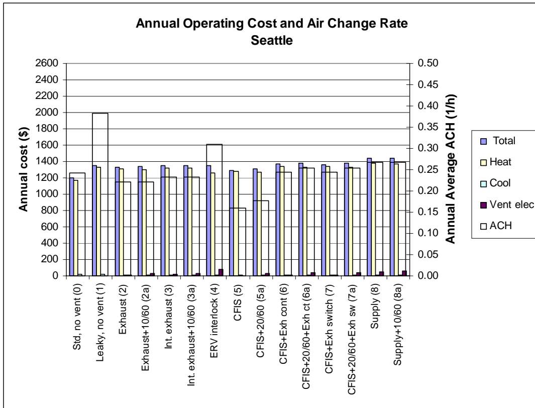
Figure B.9 Annual operating cost and annual average air change rate for Seattle
