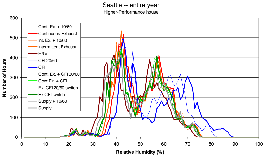
Figure B.22 Frequency distribution of hourly average indoor relative humidity (1% bins) for the entire year in Seattle
