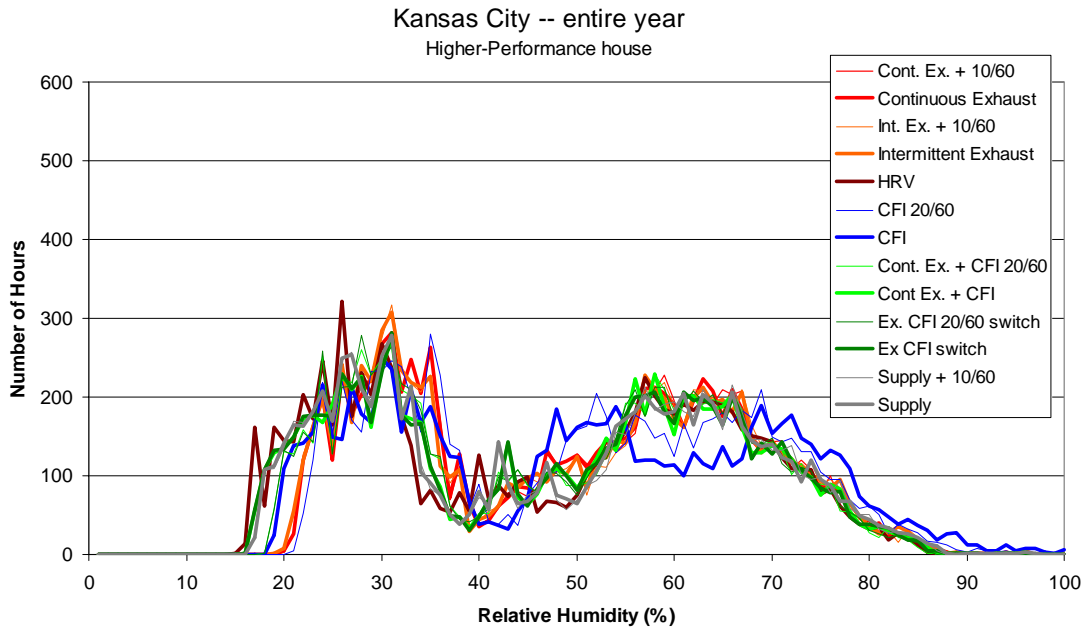
Figure B.19 Frequency distribution of hourly average indoor relative humidity (1% bins) for the entire year in Kansas City
