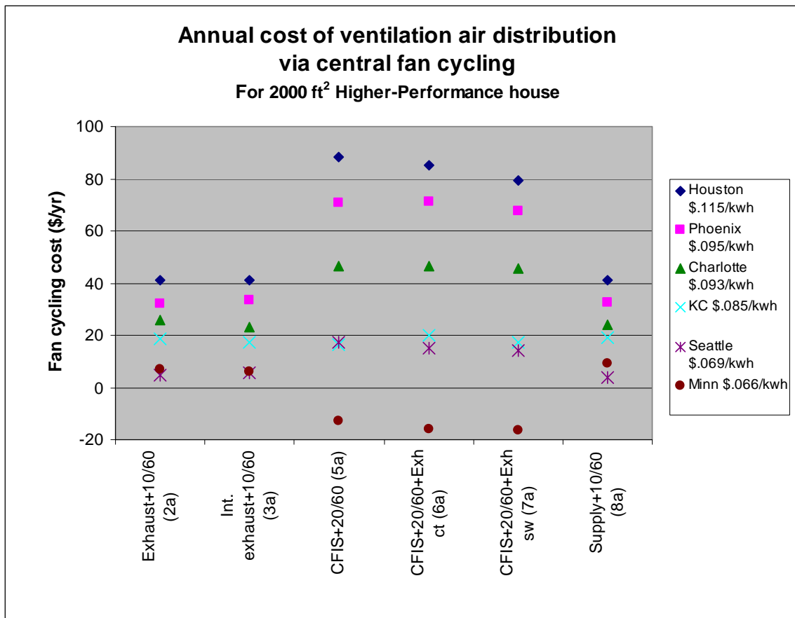
Figure 3.9(b) Annual cost of ventilation air distribution and thermal comfort mixing via the central fan for the Higher-Performance house, for all six climate locations
