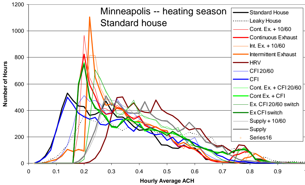
Figure A.42 Frequency distribution of hourly average air change rate (0.02 ach bins) for the heating season in Minneapolis
