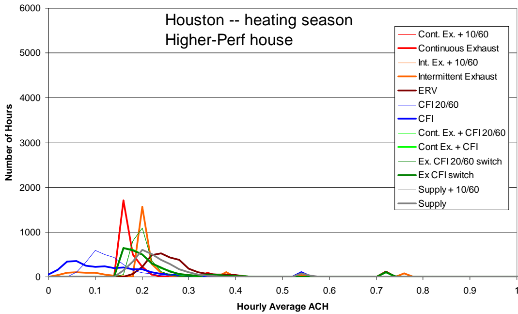
Figure B.29 Frequency distribution of hourly average air change rate (0.02 ach bins) for the heating season in Houston
