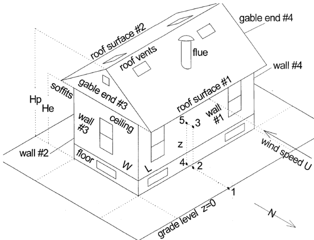
Figure C1. Illustration of house and attic airflow components
