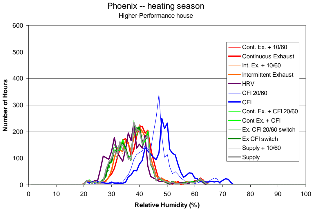
Figure B.15 Frequency distribution of hourly average indoor relative humidity (1% bins) for the heating season in Phoenix
