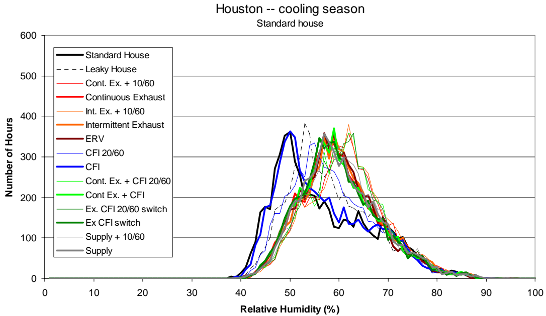
Figure 3.11(a) Frequency distribution of hourly average indoor relative humidity (1% RH bins) for the cooling season for the Standard-Performance house in Houston
