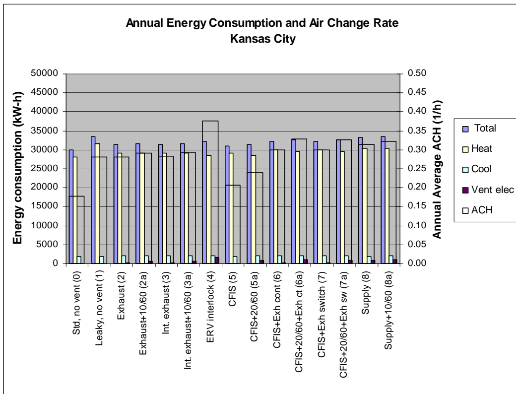
Figure A.8 Annual energy consumption and annual average air change rate for Kansas City
