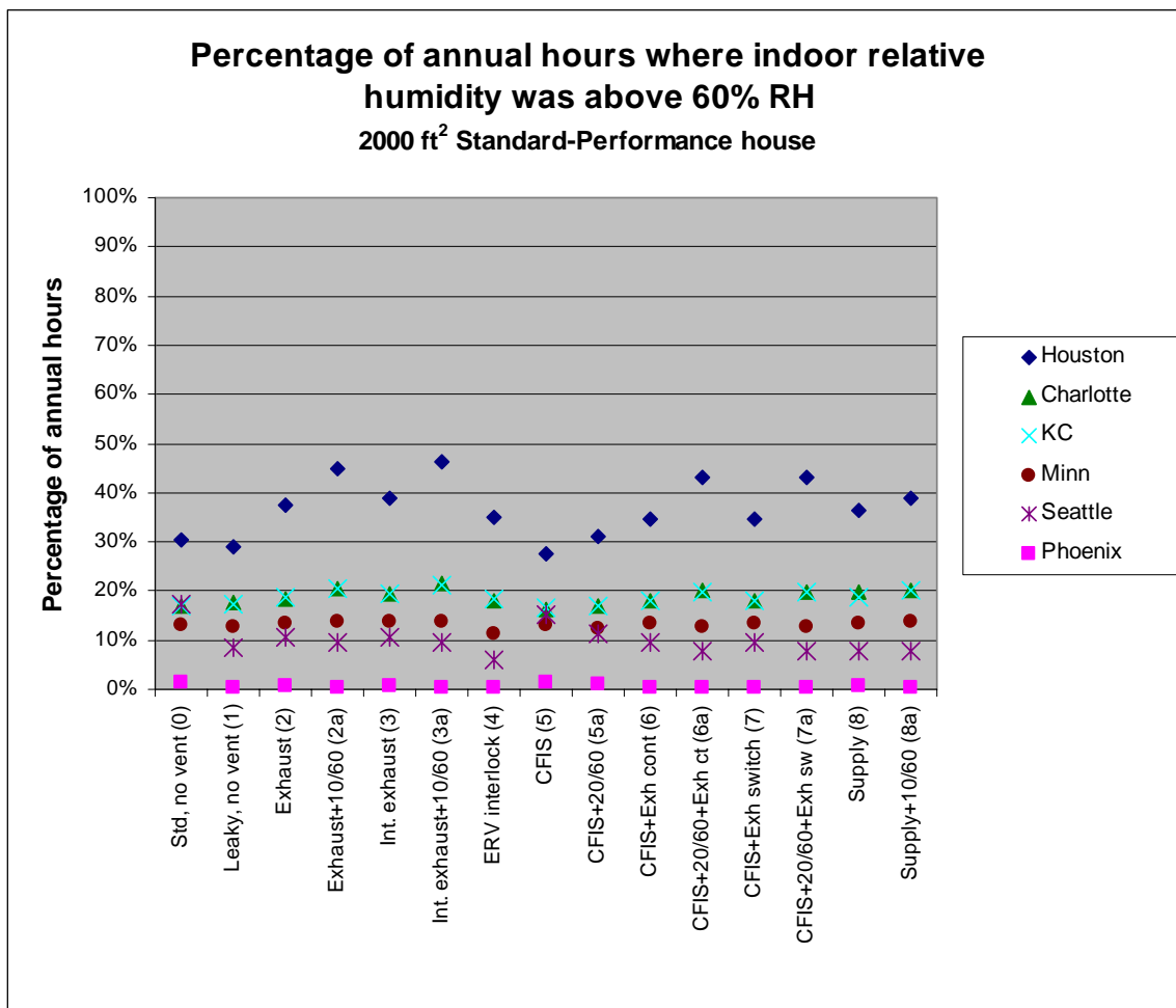
Figure 3.14(a) Percentage of annual hours where indoor relative humidity exceeded 60% RH for Standard-Performance house
