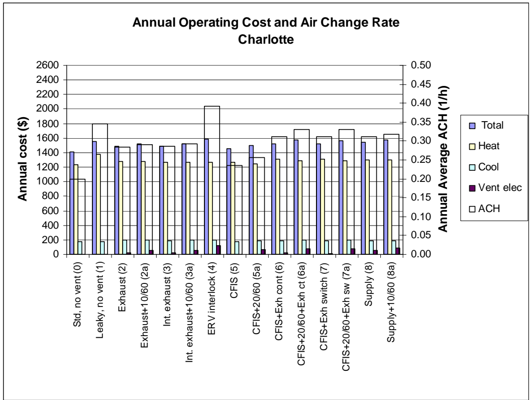
Figure A.5 Annual operating cost and annual average air change rate for Charlotte
