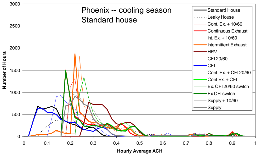
Figure A.30 Frequency distribution of hourly average air change rate (0.02 ach bins) for the cooling season in Phoenix
