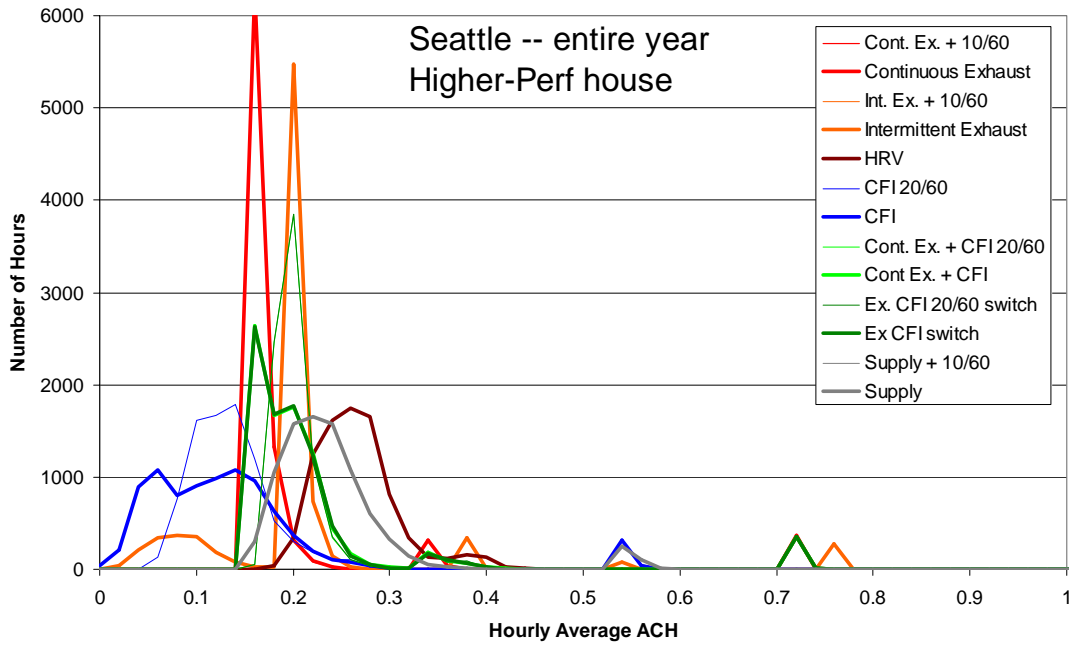
Figure 3.4(b) Hourly average air change rate (ach frequency in 0.02 bins) for Seattle, for Higher-Performance house
