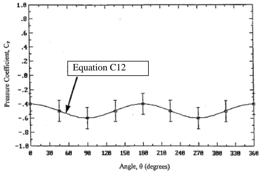
Figure C5. Roof pressure coefficients for a moderate sloped roof (10° < pitch < 30°)
