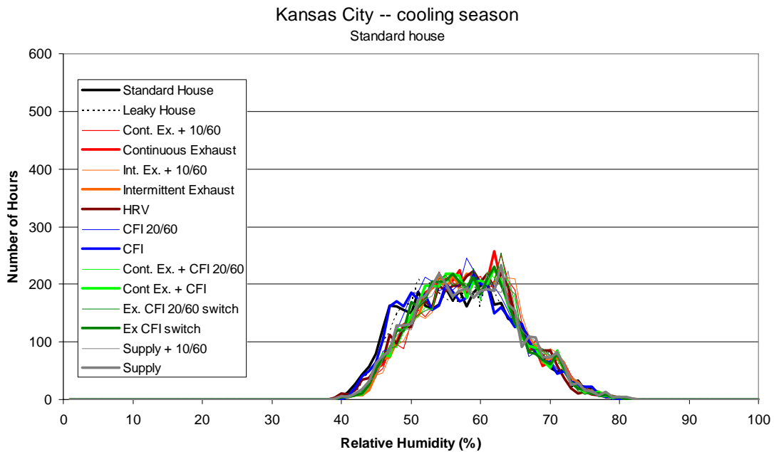
Figure A.20 Frequency distribution of hourly average indoor relative humidity (1% bins) for the cooling season in Kansas City
