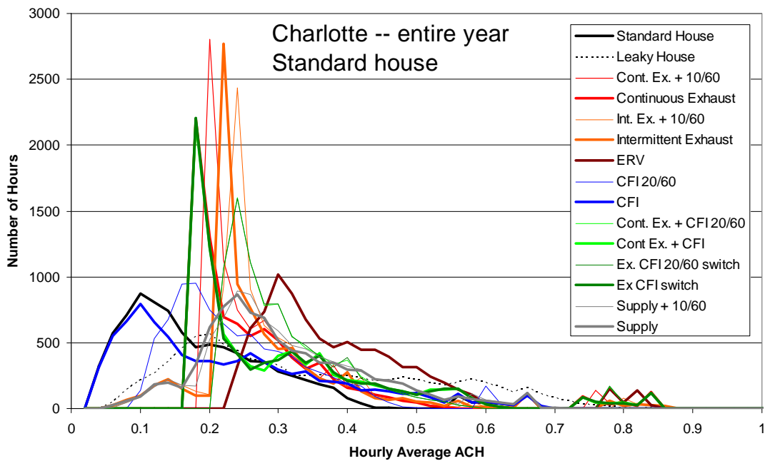
Figure A.32 Frequency distribution of hourly average air change rate (0.02 ach bins) for the entire year in Charlotte
