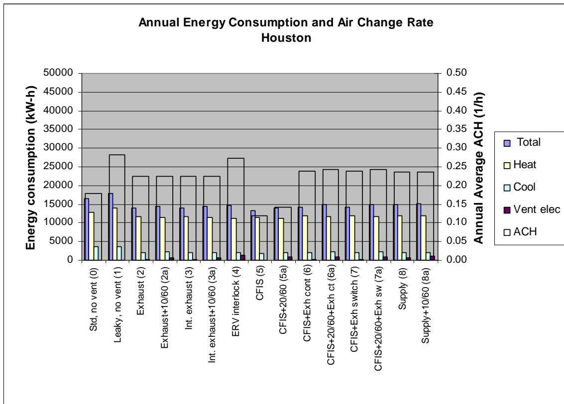
Figure B.2 Annual energy consumption and annual average air change rate for Houston
