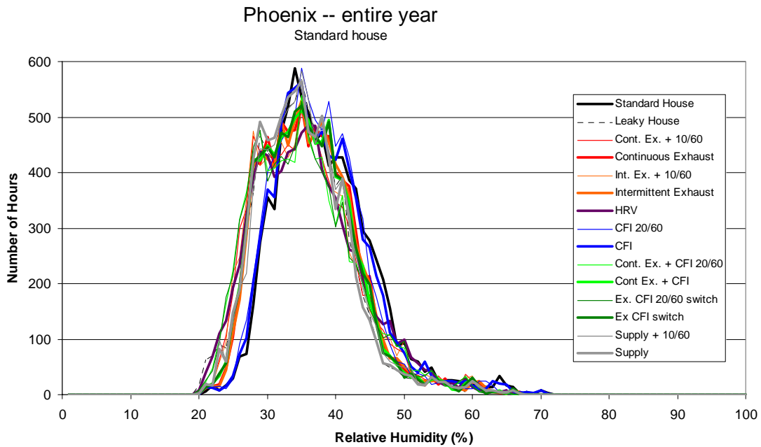
Figure A.13 Frequency distribution of hourly average indoor relative humidity (1% bins) for the entire year in Phoenix
