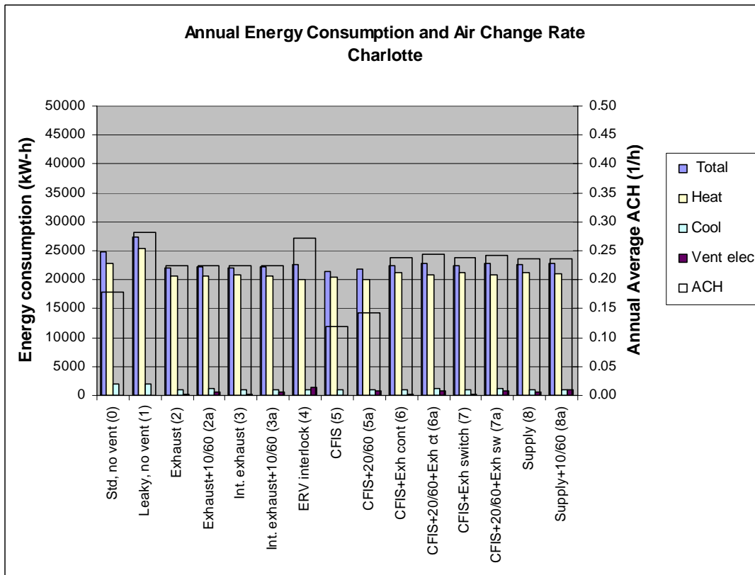
Figure B.6 Annual energy consumption and annual average air change rate for Charlotte
