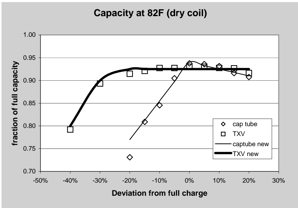
Figure C12. Dry Coil capacity variation with charge
