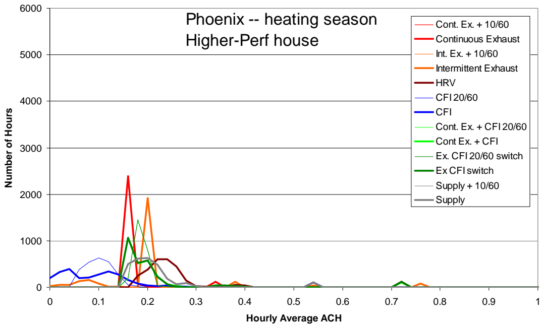
Figure B.31 Frequency distribution of hourly average air change rate (0.02 ach bins) for the heating season in Phoenix
