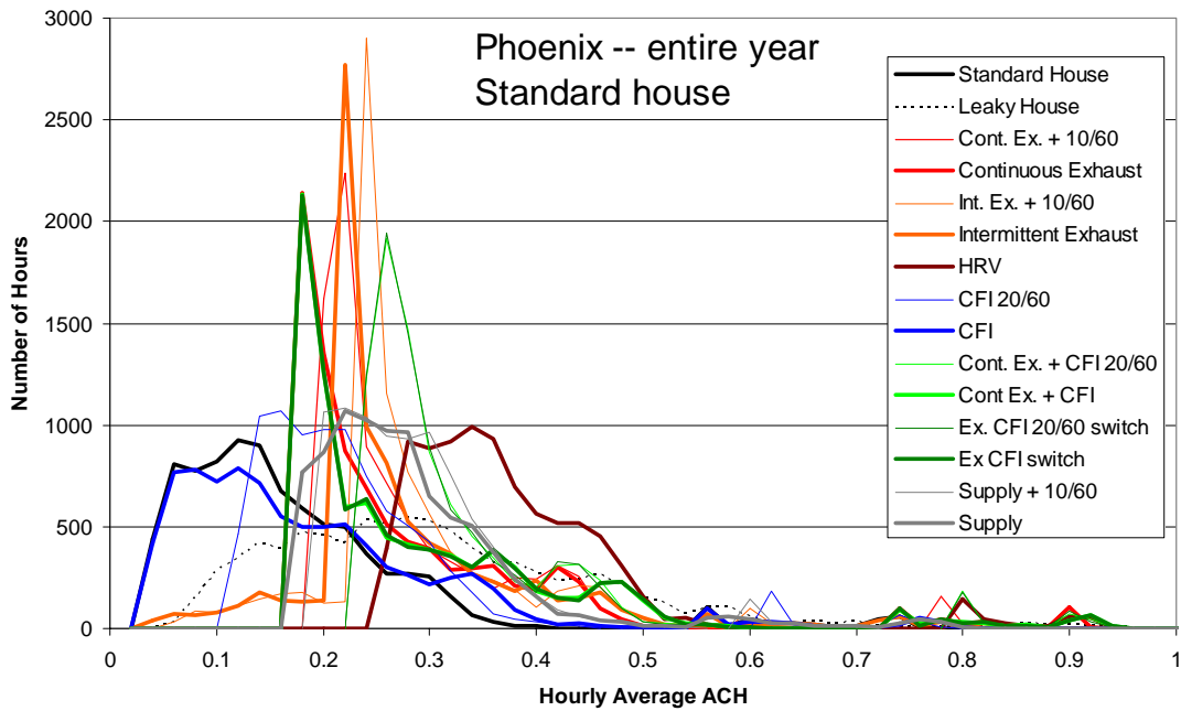
Figure 3.3(a) Hourly average air change rate (ach frequency in 0.02 bins) for Phoenix, for Standard-Performance house
