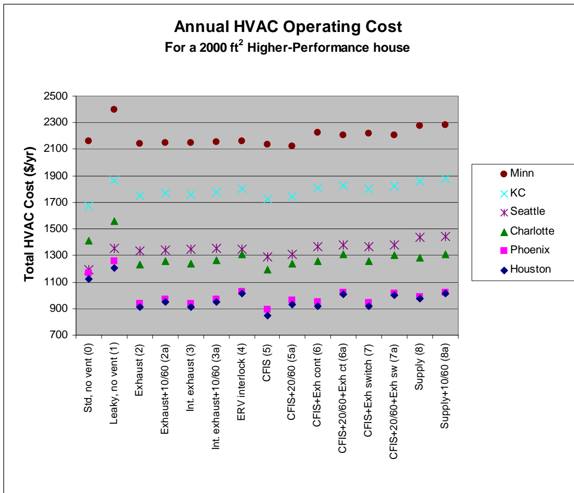
Figure 3.5(b) Comparison of annual HVAC operating cost (heating, cooling, and ventilation) for the Higher-Performance house, for all six climate locations
