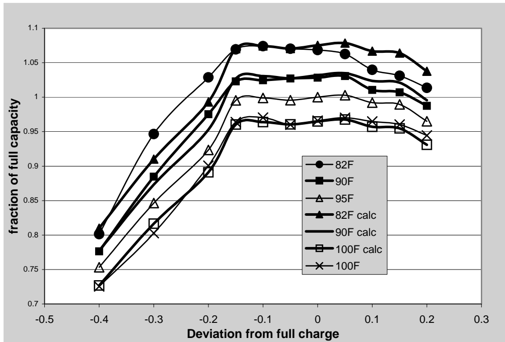
Figure C14. Dry Coil capacity variation with outdoor temperature
