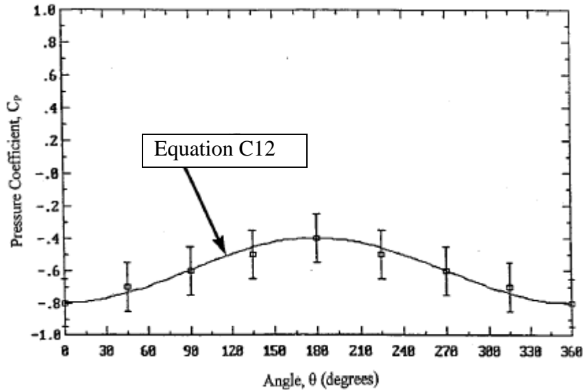
Figure C6. Roof pressure coefficients for a low sloped roof (pitch < 10°)
