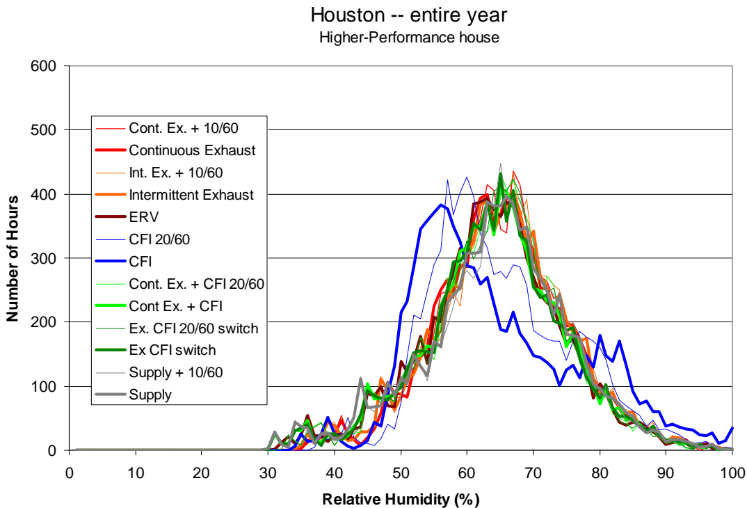
Figure 3.10(b) Frequency distribution of hourly average indoor relative humidity (1% RH bins) for the entire year for the Higher-Performance house in Houston
