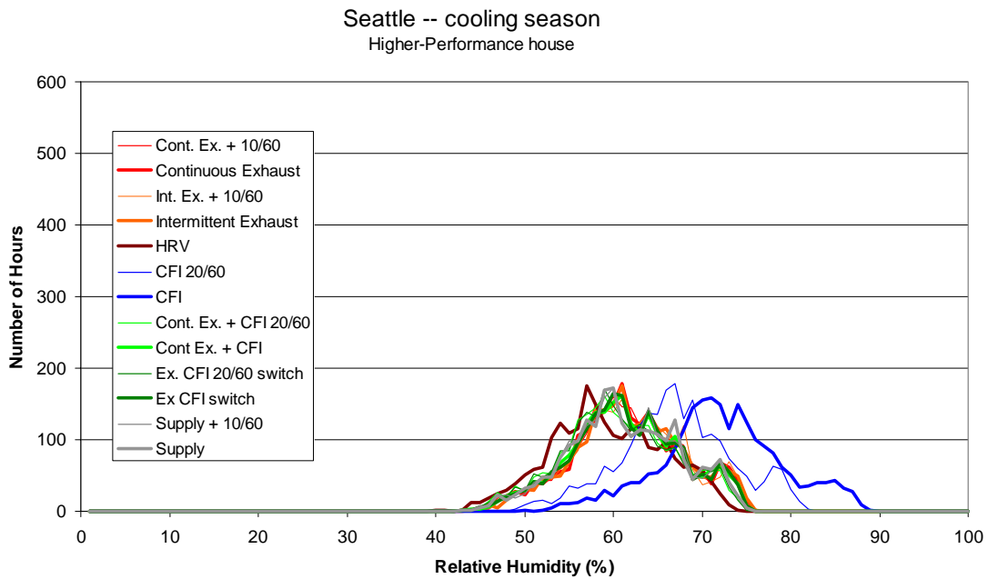
Figure B.23 Frequency distribution of hourly average indoor relative humidity (1% bins) for the cooling season in Seattle
