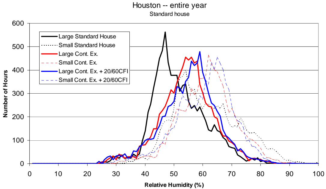
Figure 3.17 Frequency distribution of hourly average indoor relative humidity (1% bins) for large and small houses, for the Standard-Performance house in Houston
