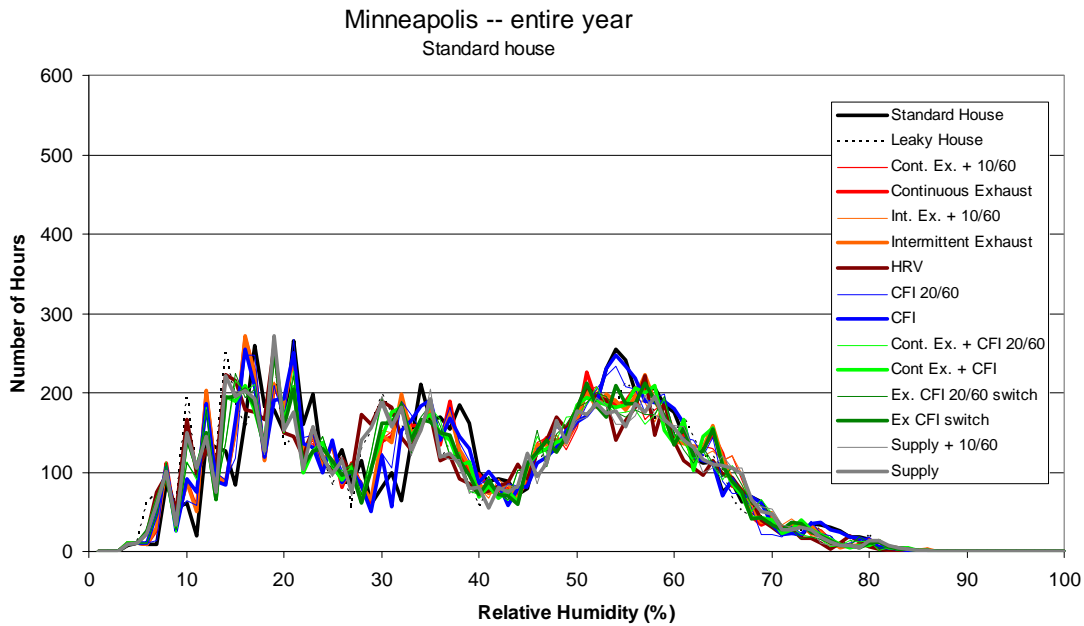
Figure 3.13(a) Frequency distribution of hourly average indoor relative humidity (1% RH bins) for the entire year for the Standard-Performance house in Minneapolis
