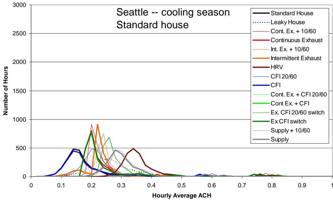
Figure A.38 Frequency distribution of hourly average air change rate (0.02 ach bins) for the cooling season in Seattle
