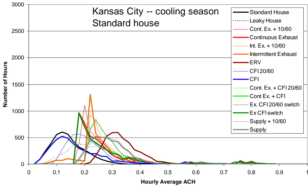
Figure A.36 Frequency distribution of hourly average air change rate (0.02 ach bins) for the cooling season in Kansas City
