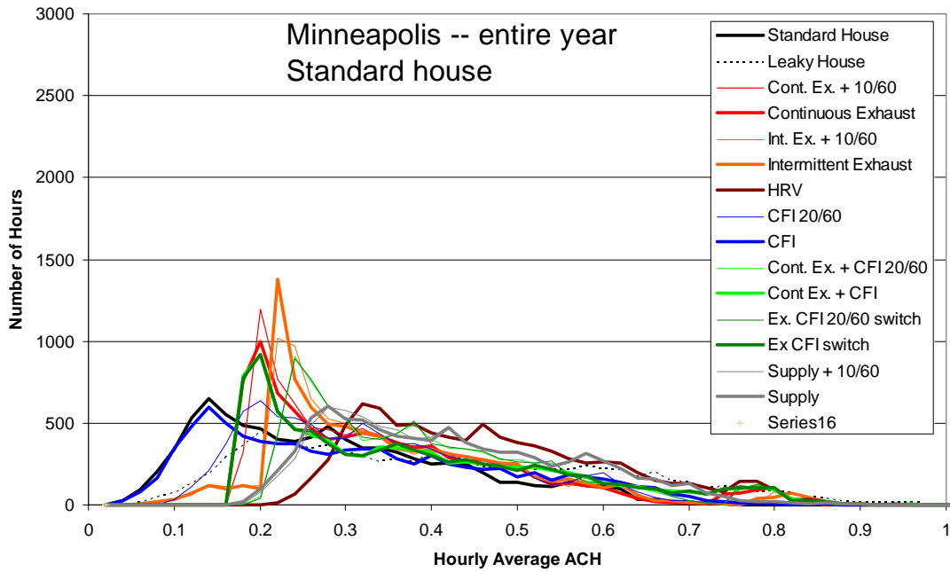
Figure A.40 Frequency distribution of hourly average air change rate (0.02 ach bins) for the entire year in Minneapolis
