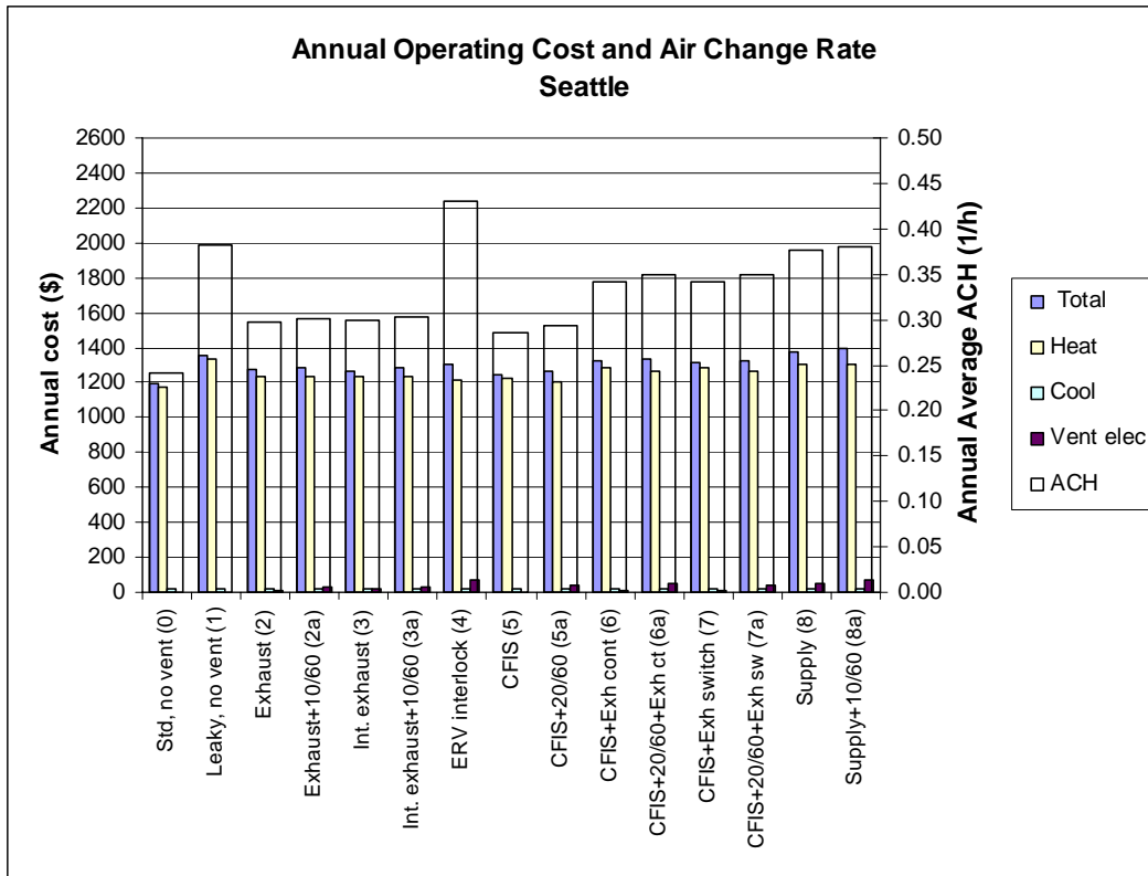
Figure A.9 Annual operating cost and annual average air change rate for Seattle
