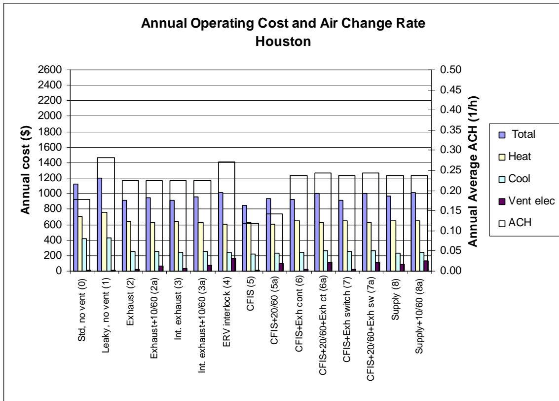
Figure B.1 Annual operating cost and annual average air change rate for Houston
