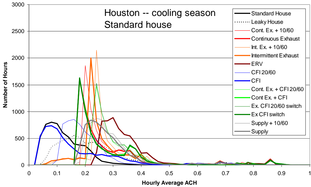
Figure A.28 Frequency distribution of hourly average air change rate (0.02 ach bins) for the cooling season in Houston
