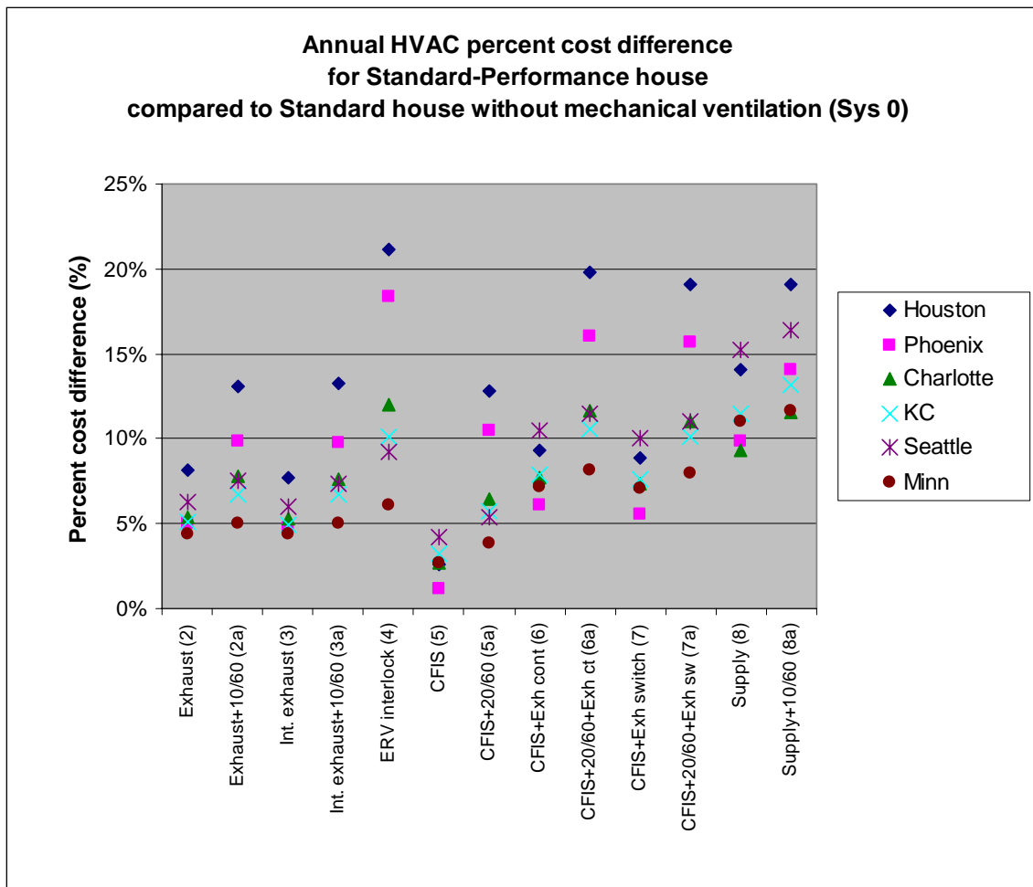
Figure 3.8(a) Annual HVAC percent cost difference for Standard-Performance house compared to the Standard house without mechanical ventilation (System 0), for all six climate locations
