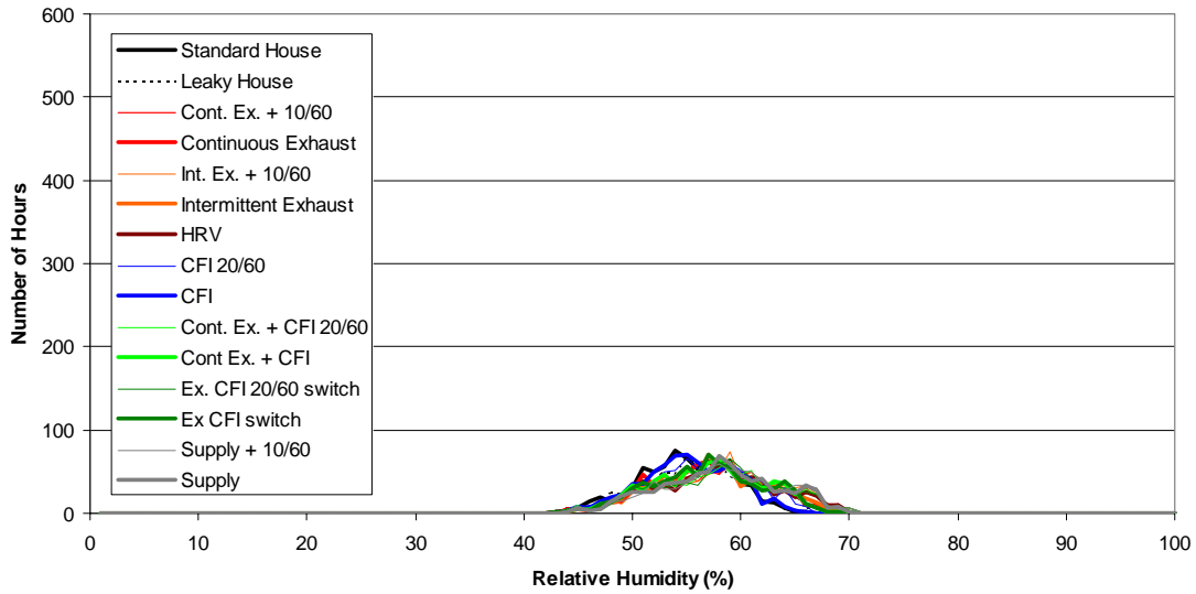
Figure A.25 Frequency distribution of hourly average indoor relative humidity (1% bins) for the cooling season in Minneapolis
