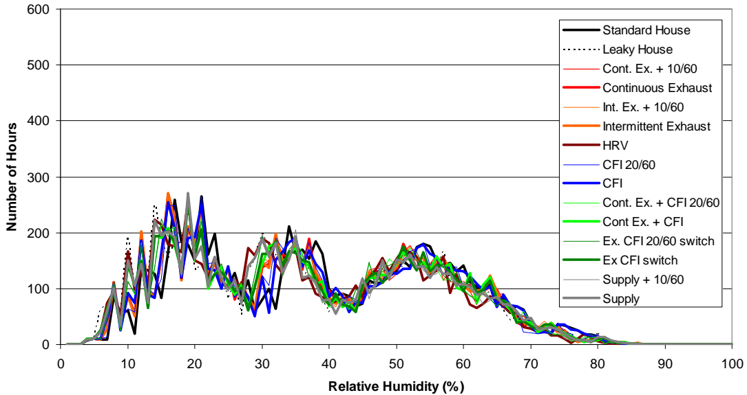
Figure A.26 Frequency distribution of hourly average indoor relative humidity (1% bins) for the heating season in Minneapolis
